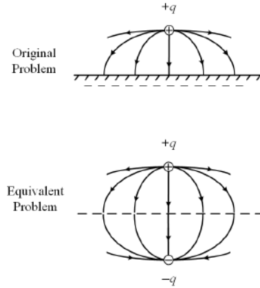
Figure 32.8: By image theory, the total electric field of the original problem and the equivalent problem when we add the total electric field due to the original charge and the image charge. It is to be noted that if we take the top half of the bottom figure, it is equivalent to the field of the top figure. The field for the bottom figure is easily obtained by superposing the fields of two opposite charges symmetrically.
