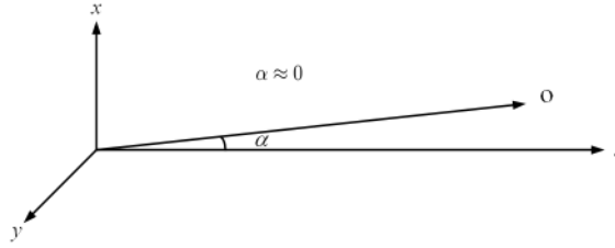
Figure 33.6: This figure shows when the paraxial approximation can be made. The wave physics are different when the field is being observed very close to the z -axis and far from it.
