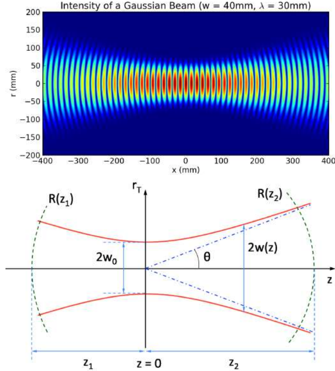
Figure 33.7: The upper figure is a more colorful one (Figure by: https://en.wikipedia.org ). Notice that these are homogeneous solutions to the wave equation since the right-hand side is always zero. The lower figure is from Glytsis [148]. Notice that the waist of the Gaussian beam, w(z) , and the radius of curvature, R(z) are functions of z . The waist at its narrowest value is w_0 = w(0) .
