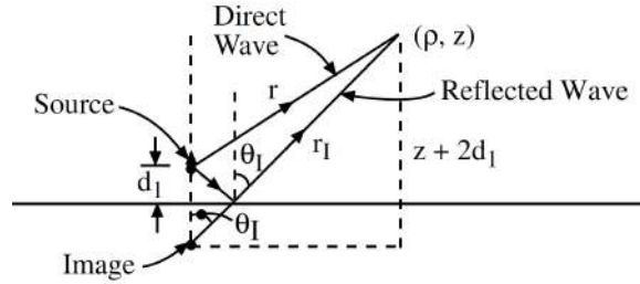
Figure 35.8: At high frequencies, the source point and the observation point are connected by a ray. The ray represents a bundle of plane waves that interfere constructively. This is even true for a bundle of plane waves that reflect off an interface. So ray theory or ray optics prevails here, and the ray bounces off the interface according to the reflection coefficient of a plane wave impinging at the interface with \theta_I .
