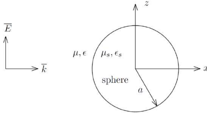
Figure 27.3: A plane electromagnetic wave incident on a particle. When the particle size is small compared to the wavelength, electrostatic analysis can be used to solve this problem (Figure by J. A. Kong [35]).
