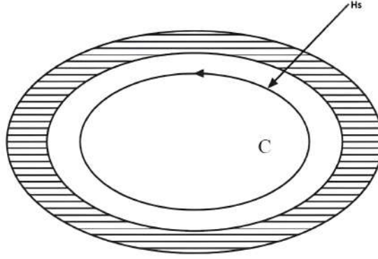
Figure 22.1: The absence of a TEM mode in a hollow waveguide enclosed by a PEC wall. The magnetic field lines form a closed loop inside the waveguide due to the absence of magnetic charges.
