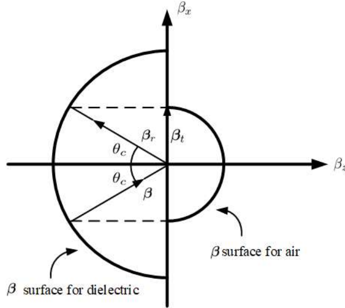
Figure 18.5: Phase-matching diagram for the total internal reflection case. Wavenumber surfaces in two regions show the phase-matching condition. In this case, the wavenumber in medium t is smaller than the wavenumber in medium 1. The figure shows an incident wave vector coming in at the critical angle. Then the transmitted wave vector is parallel to the interface as shown with \beta_z = 0 . When the incident angle is larger than the critical angle, \beta_z becomes an imaginary number as the wave vector in region t is complex and cannot be drawn.
