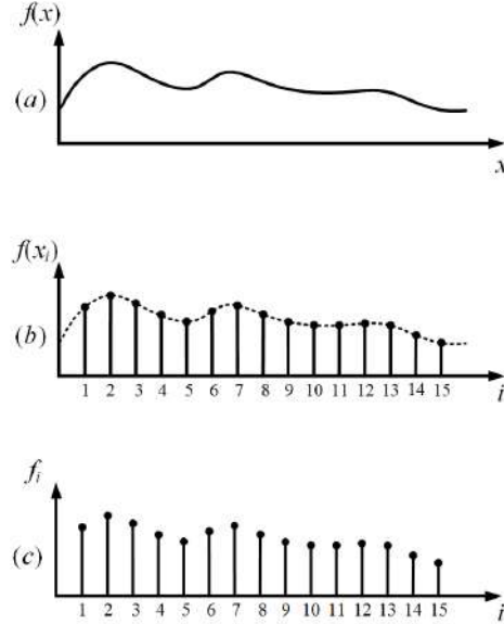
Figure 36.5: A function can be thought of as a vector. (a) A continuum function f(x) plotted as a function of x . (b) Digitally sampled values of the same function. (c) When stored in a computer, it will be stored as an array vector.
