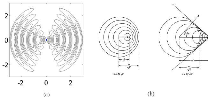
Figure 29.1: (a) Electric field around a time-oscillating dipole (Figure by physics stack exchange). (b) Equipotential lines around a moving charge that gives rise to Cherenkov radiation (Figure by J.D. Jackson [50]). We will not study Cherenkov (Cerenkov) radiation in this course, but it is written up in [35] and [50]. Its discovery and its explanation led to a Nobel Prize.
