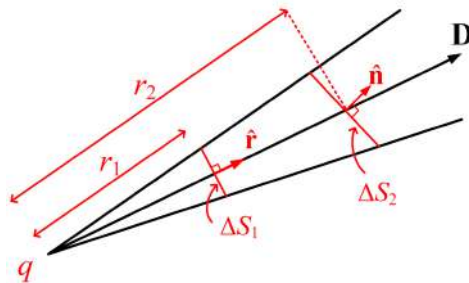
Figure 1.10: When a sliver of angular sector is taken, the same amount of electric flux from a point charge passes through two incremental surfaces \Delta S_1 and \Delta S_2 at different distances from the point charge.
