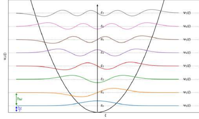
Figure 38.5: Plots of the eigensolutions of the simple quantum pendulum in normalized coordinate \xi . The photon-number states, \Psi_n(\xi) , (also called Fock state), are nonclassical states because they do not have a classical analogue. This 1D pendulum describes many dipolar oscillators in nature: the vibration of an atom in a lattice, an atom bound to a molecule, electron-hole pair, an electron sitting in a lattice, or possibly, electron-positron pairs in a vacuum.
