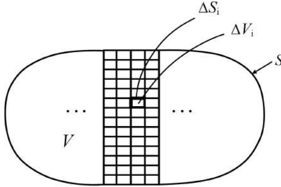
Figure 2.1: The discretization of a volume V into a sum of small volumes \Delta V_i , each of which is a small cuboid. a staircasing error occurs near the boundary of the volume V , but the error diminishes as \Delta V_i \rightarrow 0 .
