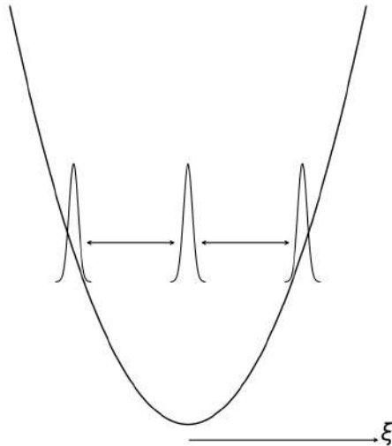
Figure 39.1: The time evolution of the coherent state. It is a wave packet that follows the motion of a classical pendulum or harmonic oscillator albeit with some uncertainty about its position.
