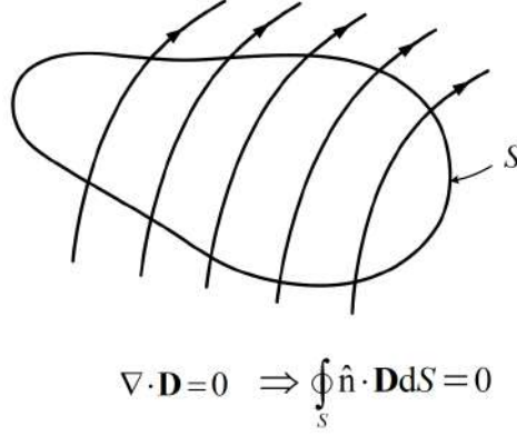
Figure 2.4: In an incompressible flux flow, flux is conserved: whatever flux enters a volume V must leave the volume V .
