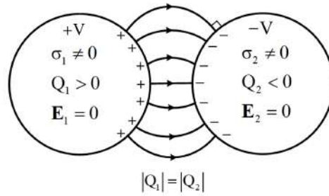
Figure 14.11: The capacitance between two charged conductors can be found by solving a BVP involving Laplace's equation as discussed in 3.3.5. If the conductors are odd shapes, then numerical methods are needed.
