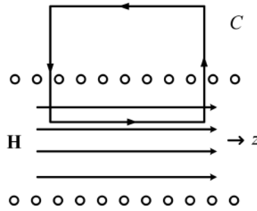
Figure 14.9: Finding the inductor flux linkage approximately by assuming the magnetic field is uniform inside a long solenoid. This approximation is more accurate as the solenoid becomes longer.
