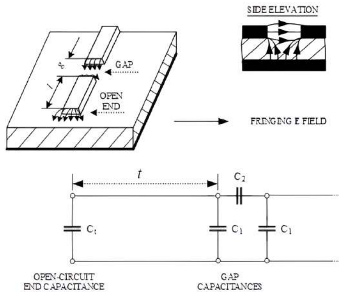
Figure 25.11: End effects and junction effects in a microwave integrated circuit are important [190, 191] (Figure by Microwave Journal). The fringing fields at the end of a microstrip line or between two microstrip lines can be modeled with parasitic capacitances. The reduction of a complex microwave circuit to a simple lumped-element approximation is a process known as parameter extraction.
