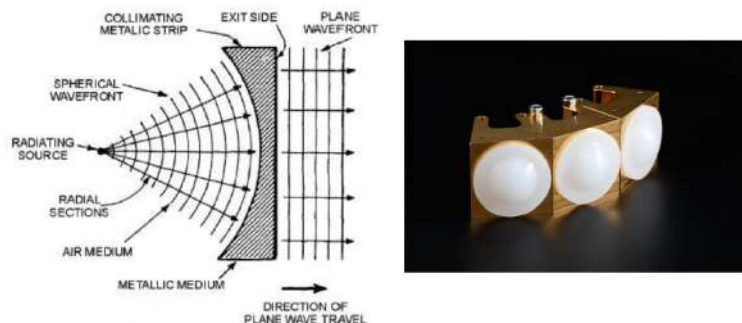
Figure 31.11: The left figure shows a lens antenna where the lens is made of artificial dielectrics made from metallic strips (Figure by: electriciantutoring.tpub.com). The right figure shows some dielectric lenses at the aperture of an open waveguide to focus the microwave exiting from the waveguide opening (Figure by: micro-radar.de). When the wavelength is much smaller than the size of the structure, a wave behaves like a ray, and quasi-optical concepts can be used to design the antenna.
