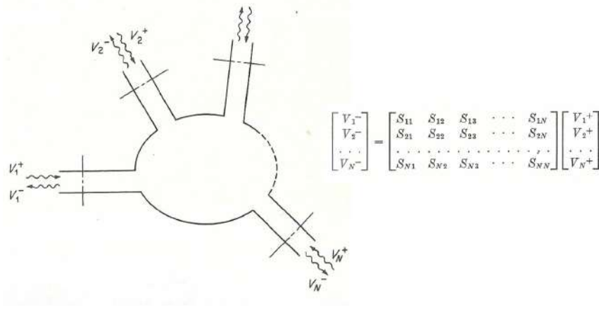
Figure 17.9: A multiport network can be characterized by its scattering matrix and the scattering parameters. Once known, microwave circuits can be concatenated together to form larger complex circuits. If the scattering parameters are known over a broad bandwidth, the behavior of the circuit in the time domain can also be obtained by Fourier transform (Figure by: Collin [104]).
