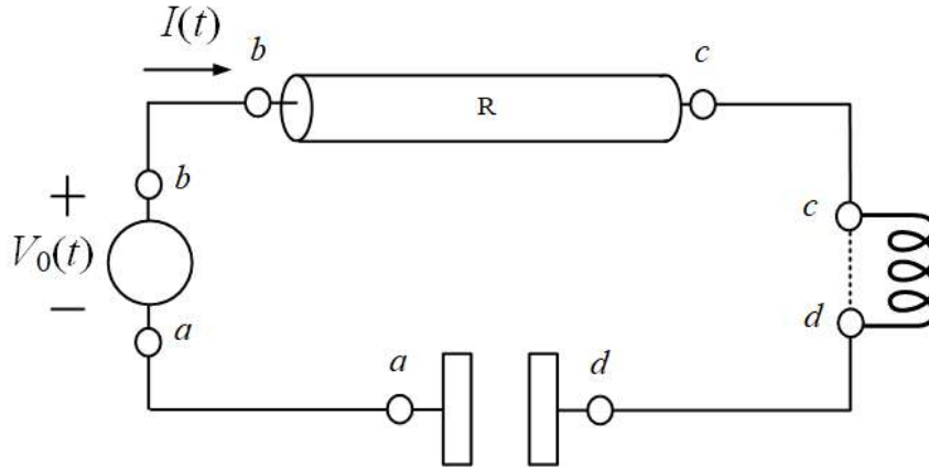
Figure 14.5: The KVL for a circuit loop consisting of resistor, inductor, and capacitor can also be derived from Faraday's law at low frequency. The KVL can be derived by integrating Faraday's law around the loop defined by abcd a . This loop does not have any magnetic flux linkage. But the detail of V_{cd} and how it relates to the flux linkage in the inductor is discussed in the text. At low frequency, the flux linkage term in Faraday's law, and the displacement current term in the generalized Ampère's law are less important, unless their effects can be amplified by using inductors and capacitors. Thus the full glory of Maxwell's equation is not lost in circuit theory (redrawn from original Figure 4.2 in Ramo et al.) [34].
