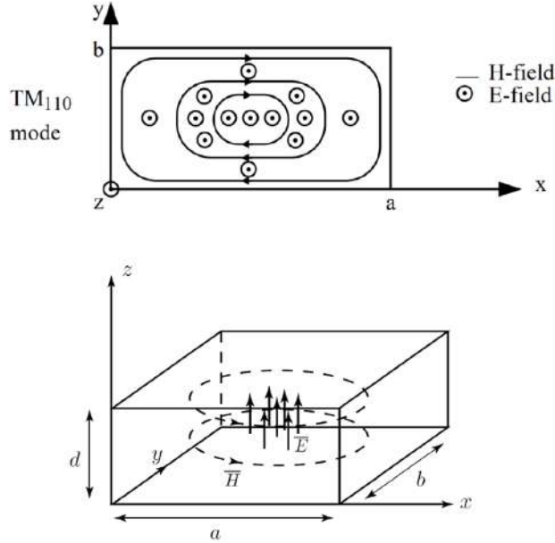
Figure 25.7: The top and 3D views of the \mathbf{E} and \mathbf{H} fields of the \text{TM}_{110} mode of a rectangular resonant cavity. Since this is a snapshot view of two sinusoidal fields that are 90 degrees out of phase, the relative signs of \mathbf{E} and \mathbf{H} fields are immaterial.
