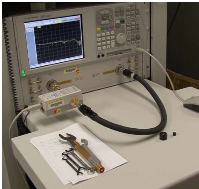
Figure 16.9: Microwave metrology technologies have progressed by leaps and bounds. I had to use a slotted line to measure the impedance of a device when I was a student. Now, a vector (measures both phase and amplitude) automated network analyzer is used and shown. It makes the measurements of microwave parameters a lot easier (Figure by: NIST).
