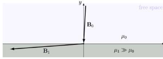
Figure 32.12: At the interface between free space and a high- \mu material, one can see that magnetic field in the free-space region is almost normal to the surface in order for normal \mathbf{B} and tangential \mathbf{H} to be continuous. Hence, looking from the free-space side, the high- \mu material resembles a PMC.
