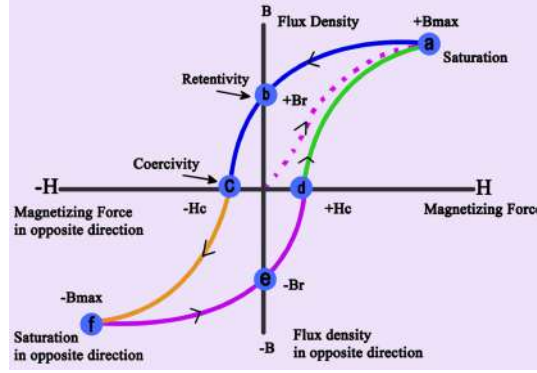
Figure 7.3: In an electric machine, the relation between the \mathbf{B} flux and the magnetic \mathbf{H} is usually nonlinear, as shown in the picture. Moreover, the nonlinear system is not time reversible, yielding a \mathbf{B} - \mathbf{H} relation as shown (Figure by: https://electricalacademia.com/electromagnetism/hysteresis-loop-magnetization-curve/ ).
