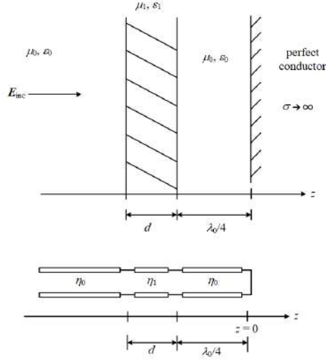
Figure 20.2: The equivalence of a layered medium problem to a transmission line problem. This equivalence is possible even for oblique incidence where a wave impedance is defined as in the previous lecture. The wave impedance is analogous to the characteristic impedance of a transmission line. For normal incidence, the wave impedance defined in the previous lecture becomes an intrinsic impedance (Figure by J.A. Kong, Electromagnetic Wave Theory ).
