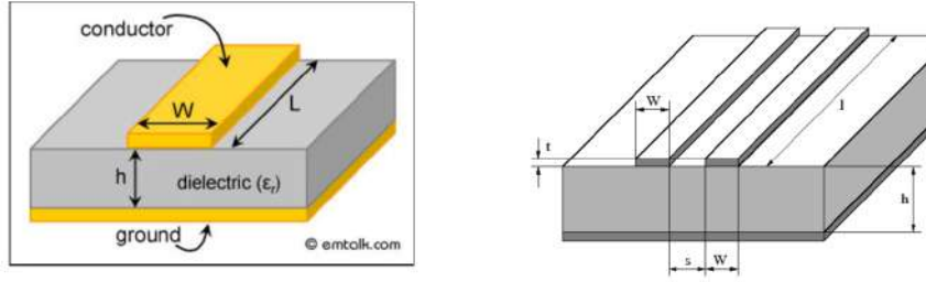
Figure 17.6: (Left) Schematic of a microstrip line with the signal line above and a ground plane below. (Right) A strip line with each strip carrying currents of opposite polarity. A ground plane is not needed in the second case. Unlike the coaxial transmission line, there is no closed-form solution for these geometries. Thanks to efficient computational electromagnetics (CEM) algorithms, numerical solutions to these problems exist (Figure by: emtalk.com, qucs.sourceforge.net).
