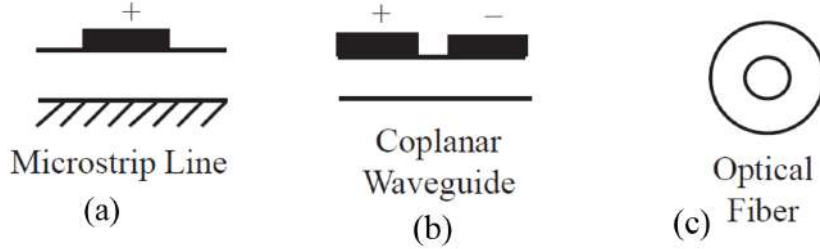
Figure 24.6: Some examples of practical coaxial-like waveguides are a microstrip line and a coplanar waveguide (left). For the microstrip line (a), the signal line (denoted with a + sign) mimics the center conductor of a coax, while the ground plane (hashed lines) represents the outer conductor of a coax. The coplanar waveguide (b) needs no ground plane and operates like a twin-ax, where the \pm line indicates the signal line and ground line of the twin-ax. The optical fiber is indicated in (c). It operates by total-internal-reflection at the interface between the center (core) of the waveguide and the cladding (outside the core). The environments of these waveguides are inhomogeneous media, and hence, a pure TEM mode cannot propagate on these waveguides.
