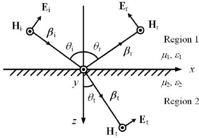
Figure 18.3: A similar schematic showing the reflection of the TM polarization wave impinging on a dielectric interface. The solution to this problem can be easily obtained from the solution for TE polarization by invoking the duality principle.
