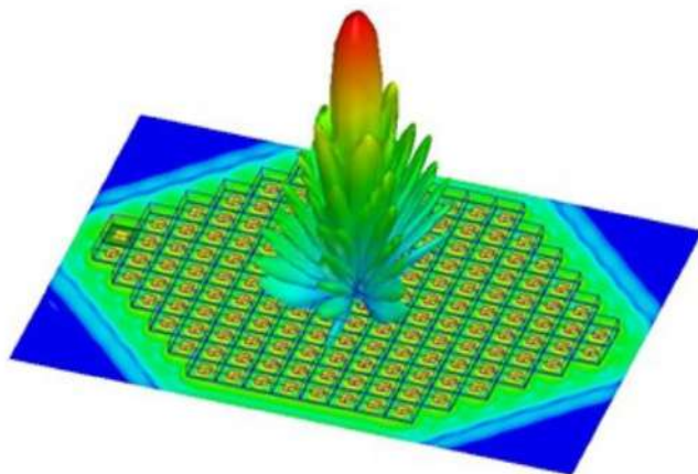
Figure 29.7: The directive gain pattern of a sophisticated array antenna for 5G applications. Presently, 5G antennas work from 24 GHz to 50 GHz, which are in the millimeter range (Figure by: Ozeninc.com).
