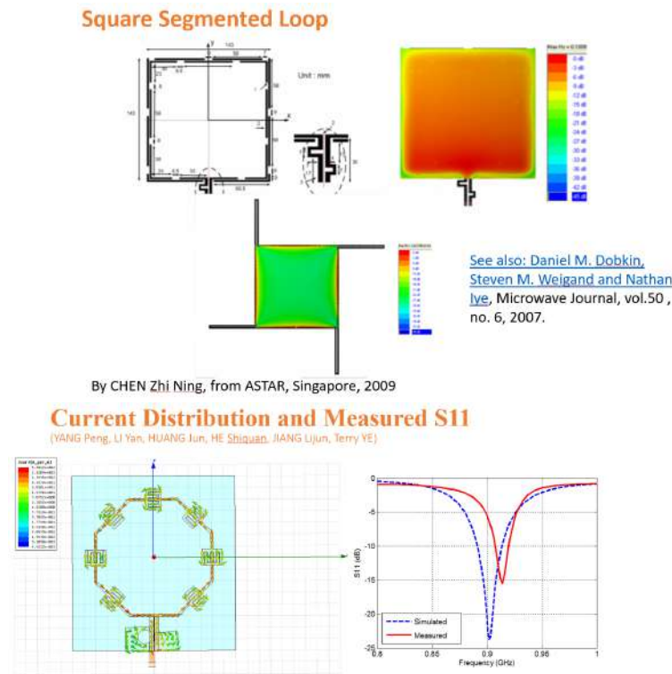
Figure 31.15: The top figure shows an RFID reader designed by [247] using a capacitively loaded inductor loop. The bottom figure shows simulation and measurement done at the University of Hong Kong and LSCM (Figure by Z.N. Chen [247] and P. Yang, Y. Li, J. Huang, L.J. Jiang, S.Q. He, T. Ye, and W.C. Chew). The series impedance is made to vanish to reduce the voltage drop across it and, hence, reduces the phase shift.
