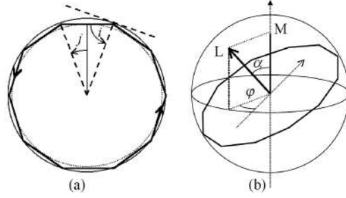
Figure 26.6: A dielectric resonator can be made by using total internal reflection of the bouncing wave within the resonator [200]. Such a mode is called a whispering gallery mode. It has high Q because the glass, from which the cavity is made, has little loss. Furthermore, the cavity can be made very large compared to wavelength, increasing the stored energy.
