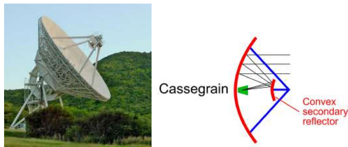
Figure 31.9: The left picture of an NRAO (National Radio Astronomy Observatory) radio telescope antenna of Cassegrain design in Virginia, USA (Figure by: Britannica.com). The right is the detail of the Cassegrain design (Figure by: rev.com). Its design is inspired by ray optics. In fact, the Cassegrain design was first used in an optical telescope.
