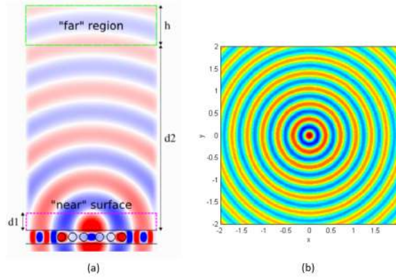
Figure 29.5: We can use numerical simulations to show the physical attributes of a spherical wave. (a) A leaky hole in a waveguide leaks a spherical wave (Figure by MEEP, MIT). (b) A point source radiates a spherical wave (Figure by ME513, Purdue Engineering). Most of these simulations are done with the FDTD (finite-difference time-domain) method that we will learn later in the course. When the wavelength is short, or the frequency high, a spherical wave looks locally like a plane wave. This is similar to the notion of humans, who are small, thinking that the earth is flat around us. To this day, some people still believe that the earth is flat:)
