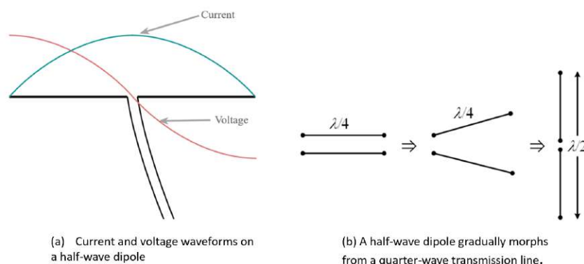
Figure 31.1: A half-wave dipole can be thought of as a resonator with radiation loss. It can be thought of as a quarter-wavelength transmission line that is gradually opened up or flared (Figure by: electronics-notes.com).
