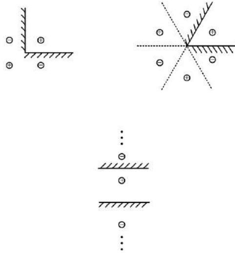
Figure 32.15: Image theory for multiple images [34].
