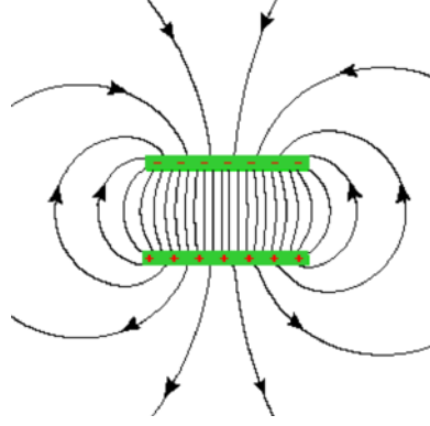
Figure 14.10: Nominally, the field in between two parallel plates in a capacitor is non-uniform. When the parallel plate is large, the ballpark value of the capacitor can be estimated by assuming a uniform field in between them. The correction to this simple formula incorporating fringing fields requires some tour-de-force analysis [117] (Figure by: https://electronics.stackexchange.com/questions/647189/what-are-changes-in-field-lines-after-two-plates-of-capacitors-are-connected ).
