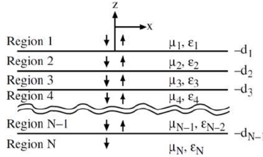
Figure 20.1: Schematic of waves in layered media. A wave entering the medium from above can be multiply reflected before emerging from the top again or transmitted to the bottommost medium.
