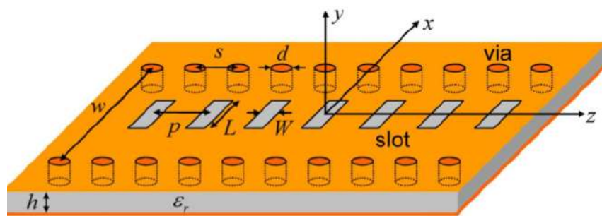
Figure 25.12: A substrate integrated waveguide from [194]. The shorting pins help to confine the fields, and they are also easily fabricated as part of the microwave integrated circuit.
