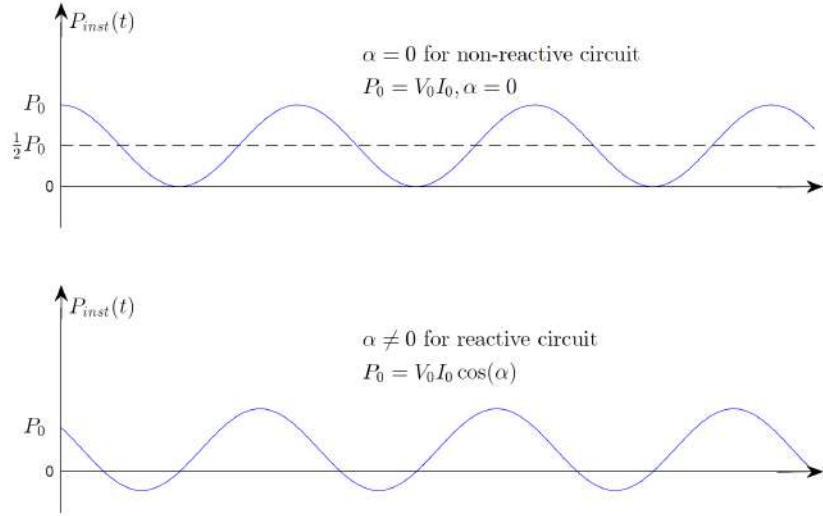
Figure 6.3: (Top) Plots of instantaneous power for when the voltage and the current is in phase ( \alpha = 0 ), and (Bottom) when they are out of phase ( \alpha \neq 0 ). In the out-of-phase case, there is an additional time-varying term that does not contribute to time-average power as shown in (6.3.15). But the instantaneous power can be negative as shown.
