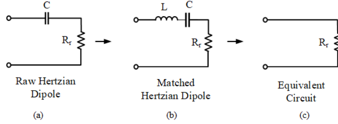
Figure 28.8: A short Hertzian dipole, shown in Figure 28.1, resembles an open circuit with a capacitor connected to it because the two spheres shown in Figure 28.1 will have charges stored in them, giving rise to electric energy stored. The radiation loss of the antenna can be modeled by a radiation resistance R_r . Hence, we have (a) an equivalent circuit of a raw Hertzian dipole without matching; (b) an equivalent circuit of a matched Hertzian dipole (using maximum power transfer theorem [57, sections 2.5 and 4.3], [125]); and (c) an equivalent circuit of a matched dipole at the resonance frequency of the LC tank circuit.
