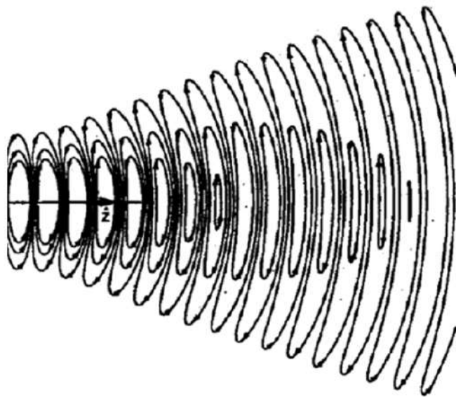
Figure 30.7: In the above figure, which is the right half of a Gaussian beam, it displays the physics of the near field, the Fresnel zone, and the far zone as one moves from the left to the right in the picture. In the far zone, the field behaves like a spherical wave (Figure by H. Haus, Electromagnetic Noise and Quantum Optical Measurements , [91]).
