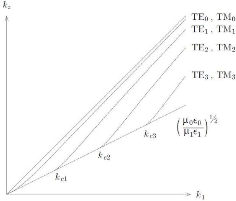
Figure 21.7: Here, we have k_z versus k_1 plots for dielectric slab waveguide. Near its cutoff, the energy of the mode is in the outer region, and hence its group velocity given by \frac{d\omega}{dk_z} is close to that of the outer region. At high frequencies, the mode is tightly bound to the slab, and its group velocity approaches that of the dielectric slab (Figure by J.A. Kong [35]).
