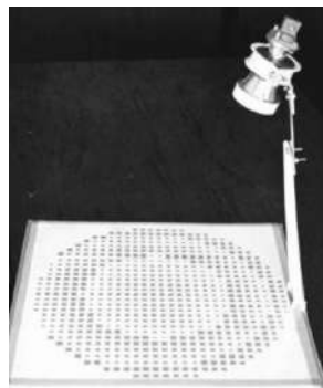
Figure 31.10: A reflectarray where the reflector is a flat surface. Patches are unequally spaced to give the array the focusing effect. No closed form solution exists for such a reflectarray, but due to advancement in computational electromagnetics (CEM), it can be simulated or virtual-prototyped in a computer (Figure by: antenna-theory.com).
