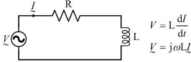
Figure 6.2: A simple circuit to illustrate the concept of complex power in circuit theory. The voltage and current are out of phase, which is a frequency-domain concept.
