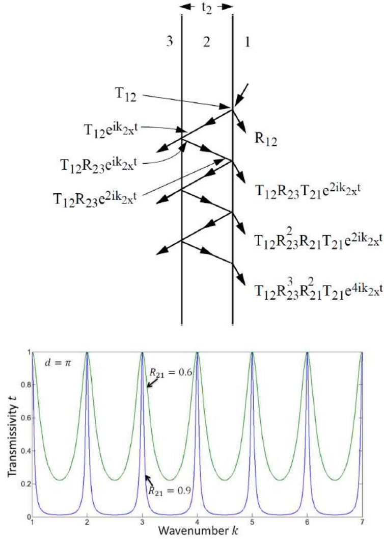
Figure 25.13: Design of a Fabry-Pérot resonator [61, 195, 92, 196]. As the magnitude of the reflection coefficient becomes close to one, the wave is better trapped inside the slab. A resonant mode exists inside the slab, providing a means for resonance tunneling.
