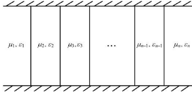
Figure 24.8: A waveguide filled with layered medium is mathematically homomorphic to a multisection transmission line problem. In this problem, there is no mode conversion and a single mode can propagate through the waveguide. And yet, the boundary conditions at the interfaces can be satisfied, like plane waves in layered media. Hence, the transmission-line method can be used to solve this problem.
