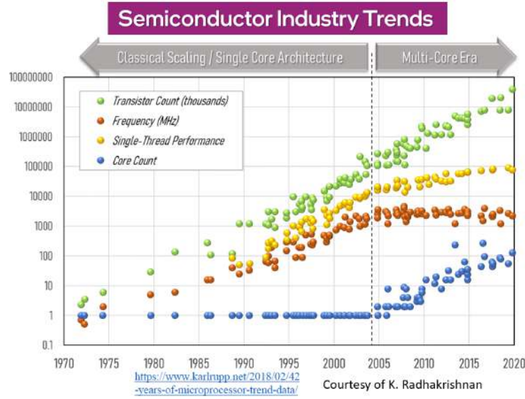
Figure 14.17: The semiconductor trends reveal the self-fulfilling prophecy of Moore's law. Ingenious engineering and 3D architecture of the microchip design allow the transistor and core counts to improve the performance of the microchip. Also, the clock rate (frequency) has not increased in the last two decades due to joule heating to be explained next. (Figure by: ieeexplore.ieee.org/document/9377004/references )
