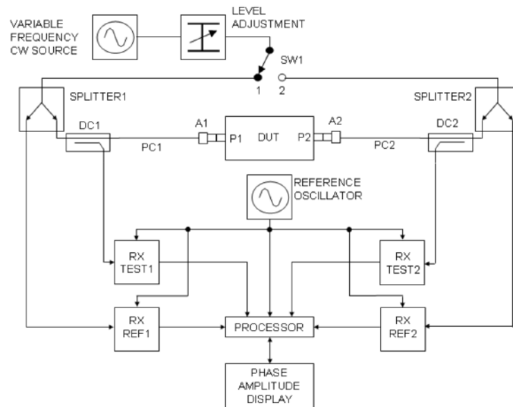
Figure 16.11: A schematic of the automated network analyzer. You can get the definitions of the acronyms from [134] (Figure by, en.wikipedia.org).
