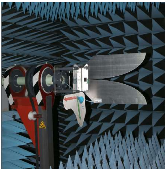
Figure 31.8: A Vivaldi antenna, also called a notched antenna, works like a horn antenna, but uses very little metal and is lightweight. Hence, it is cheap to build, and its flared notch makes it broadband. It is broadband because the high frequency signals can radiate from the narrow part of the notch, and the lower-frequency signals can radiate from the wider part of the notch (Figure by: https://en.wikipedia.org ).
