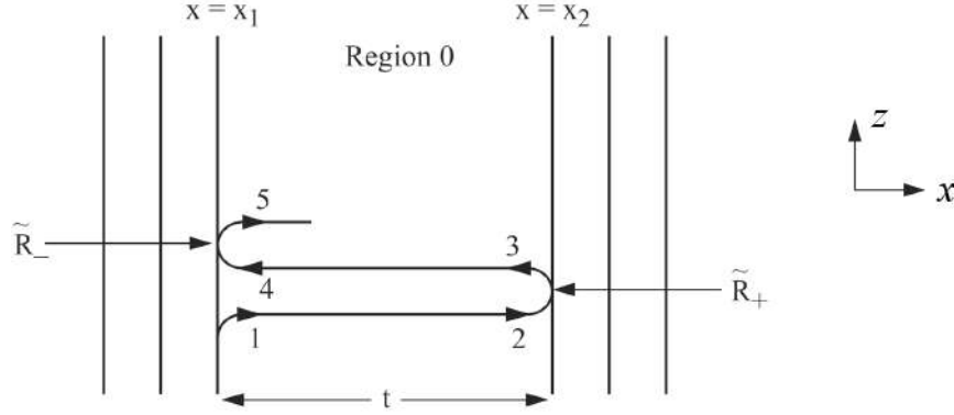
Figure 21.1: For constructive interference to occur, the phase of the wave at position 5 should be equal to the transverse phase at position 1. The above is an illustration, as the ray does not bend as shown.
