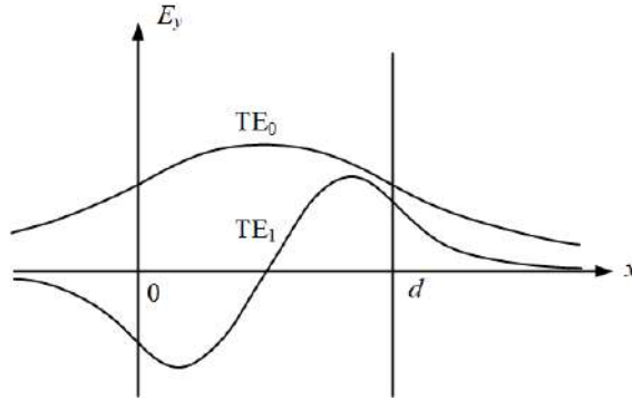
Figure 21.5: Mode profiles of the TE_0 and TE_1 modes of a dielectric slab waveguide (Figure by J.A. Kong [35]).
