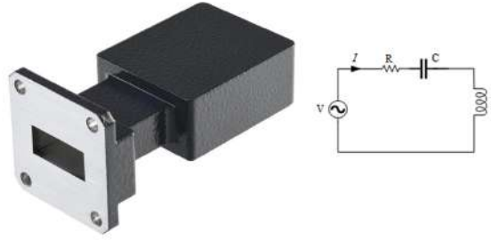
Figure 25.5: A rectangular waveguide terminating with a short at one end and an open circuit at the other end. The open end can also act as an antenna as it radiates. When the cavity is injected with electromagnetic fields coinciding with its resonance frequency, the fields inside the cavity become large, and so do the fields at the aperture, making it a better radiator. This is a cavity-backed antenna: it uses resonance tunneling to enhance its radiation capability. (Resonance tunneling phenomenon describes the ease with which photons tunnel through a barrier when the photons are close to the resonance frequency of the barrier structure). The RLC circuit can approximate the physics of the structure (Figure by RFcurrent.com).
