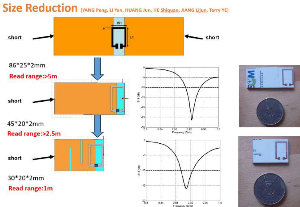
Figure 31.14: Some RFID antennas designed at the University of Hong Kong in collaboration with LSCM (Logistics and Supply Chain Multitech, R&D Center, Hong Kong). The image theory together with the use of tortuous current flow patterns are used to miniaturize the antennas (Figure by P. Yang, Y. Li, J. Huang, L.J. Jiang, S.Q. He, T. Ye, and W.C. Chew).
