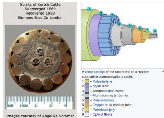
Figure 18.9: An old 1869 submarine cable made of coaxial cables (left) and modern submarine cable made of optical fibers (right) (Figure by Atlantic-Cable [151], https://en.wikipedia.org [152]). Comparing them to the optical fiber now, we have come a long way!
