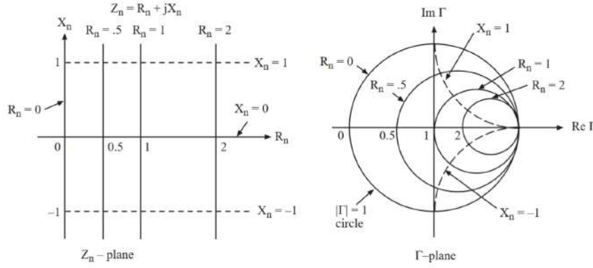
Figure 16.4: Bilinear map of the formula \Gamma = \frac{Z_n - 1}{Z_n + 1} , and Z_n = \frac{1 + \Gamma}{1 - \Gamma} . It maps circles to circles. The chart on the right, called the Smith chart, allows the values of Z_n to be determined quickly once given \Gamma , and vice versa.
