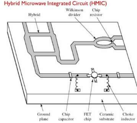
Figure 17.7: A general microwave integrated circuit with different kinds of elements (Figure by: Slideplayer.com).
