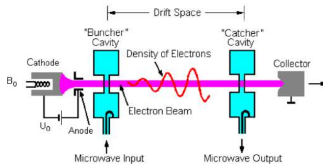
Figure 25.14: A klystron works by converting the kinetic energy of an electron beam into the energy of a traveling microwave next to the beam. As the microwave rides on the electron beam, it absorbs energy from the kinetic energy of the electrons, making its amplitude grow as it propagates. The amplified microwave can be collected by the "catcher" cavity (Figure by: https://en.wikipedia.org/wiki/Kly [197]).
