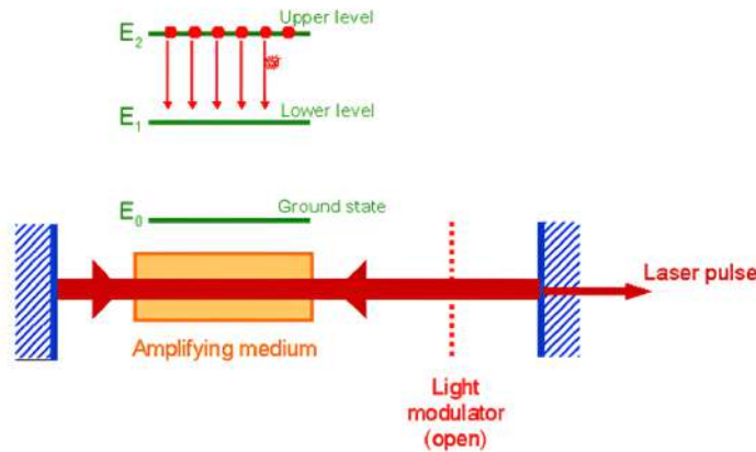
Figure 25.16: A simple view of the physical principle behind the workings of the laser. The cavity again enhances the interaction of the photons with the amplifying medium (Figure by: www.optique-ingenieur.org ).
