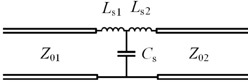
Figure 24.10: When the single-mode approximation holds, one assumes that away from the waveguide junction, there is only one single mode. Close to the waveguide junction, however, the evanescent, higher-order modes give rise to localized stored electric and magnetic energies at the waveguide junction. Circuit elements are used to account for these stored energies at the waveguide junctions. They also account for the fact that the currents and voltages are not continuous across the junctions anymore, as the fields of the dominant modes in each section (as shown in Figure 24.9) are not continuous anymore. The moral of the story is that engineers love to replace complicated theories with simple ones in order to solve complex problems.
