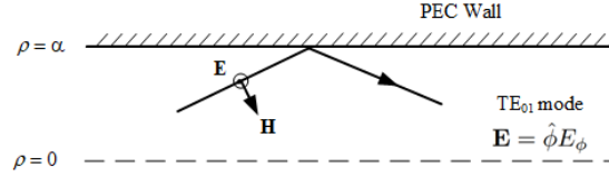
Figure 24.1: Bouncing wave picture of the Bessel wave inside a circular waveguide for the TE_{01} mode. One can also explain the low-loss physics [181] using the TE mode of a parallel-plate waveguide (see related text).
