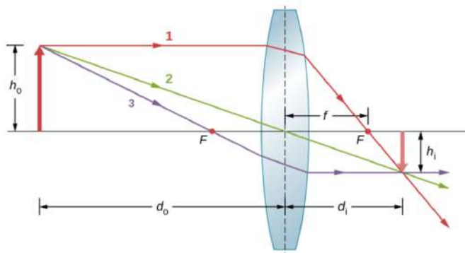
Figure 18.4: Ray tracing, based on Snell's law of refraction, can be used to solve many optics problems when the wavelength is small compared the to the size of the geometry (Figure by Steven Mellema, The Cosmic Universe).
