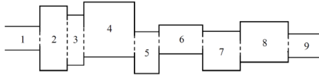
Figure 24.9: A multisection waveguide is not exactly homomorphic to a multisection transmission line problem when the cross section of the waveguides are not equal to each other. The boundary conditions at the junction cannot be met by assuming a single mode. Therefore, multimodes are needed to match the boundary conditions [96]. Circuit elements are needed at the junctions to approximately capture the physics at the waveguide junctions as shown in the next figure.
