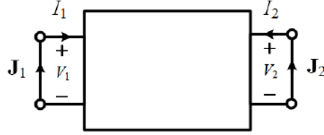
Figure 12.6: The interaction between two antennas, not necessarily in the far field of each other, can be reduced to a circuit theory description since the input and output ports of the antennas are small compared to the wavelength. But inside the box, any linear time-invariant medium can be there.
