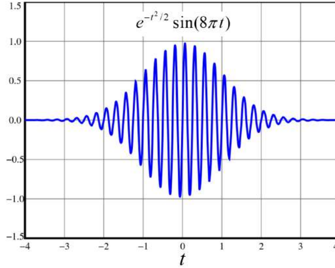
Figure 20.4: A Gaussian wave packet as a function of t for a fixed z . It can be thought of as a linear superposition of many monochromatic waves with slightly different frequencies. If one Fourier transforms the above signal, it will become a narrowband signal centered about certain \omega_0 (Figure by Wikipedia).
