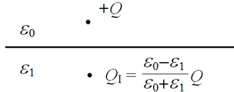
Figure 32.17: A static charge over a dielectric interface can be found in closed form using Fourier transform technique, to be discussed later. The solution is beyond the scope of this lecture at this point.
