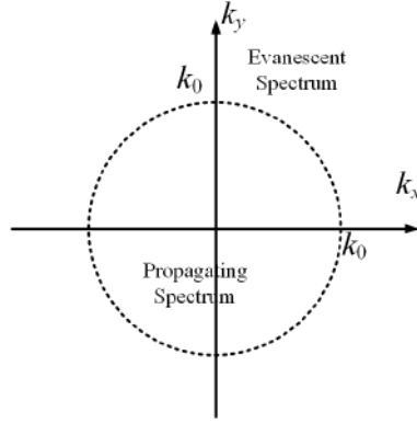
Figure 35.2: The integral in the Weyl identity is done over the entire k_x - k_y plane. The wave is propagating for \mathbf{k}_\rho = \hat{x}k_x + \hat{y}k_y vectors inside the disk, while the wave is evanescent for \mathbf{k}_\rho outside the disk. This is easily seen by the \exp(ik_z|z|) = \exp(i\sqrt{k_0^2 - k_x^2 - k_y^2}|z|) dependence of the integrand in (35.1.11). Therefore, the high spectral frequency components of the Fourier integral that is outside the disk form the evanescent spectrum.
