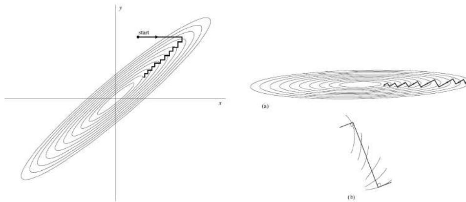
Figure 36.9: Plot of a 2D cost function, I(x, y) for an ill-conditioned system (Figure by Numerical Recipe [307]). A higher-dimensional plot of this cost function will be difficult. The zig-zag search path is the hallmark of an ill-conditioned system. This cost function has only two eigenvalues, one of which is larger than the other one.
