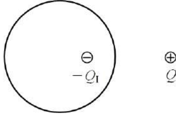
Figure 32.16: Image theory for a point charge near a cylinder or a sphere can be found in closed form. Details are given in [34].
