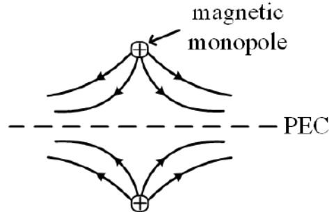
Figure 32.9: On a PEC surface, the requisite boundary condition is \hat{n} \cdot \mathbf{B} = 0 . Hence, a static magnetic monopole on top of a PEC surface will have a magnetic field distributed as shown. By image theory, such a distribution of the \mathbf{B} field can be obtained by adding a magnetic monopole of the same polarity at its image point.
