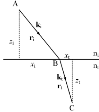
Figure 33.4: In Fermat's principle, a light ray, when propagating from point A to point C , takes the path of least time delay in the time domain, and hence, the least phase shift in the frequency domain.
