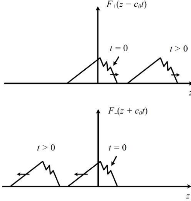
Figure 3.1: Solutions of the wave equation can be single-value functions of any shape. In the above, F_+ travels in the positive z direction, while F_- travels in the negative z direction as t increases. The pulses are delayed version of each other, and this is the retardation physics.
