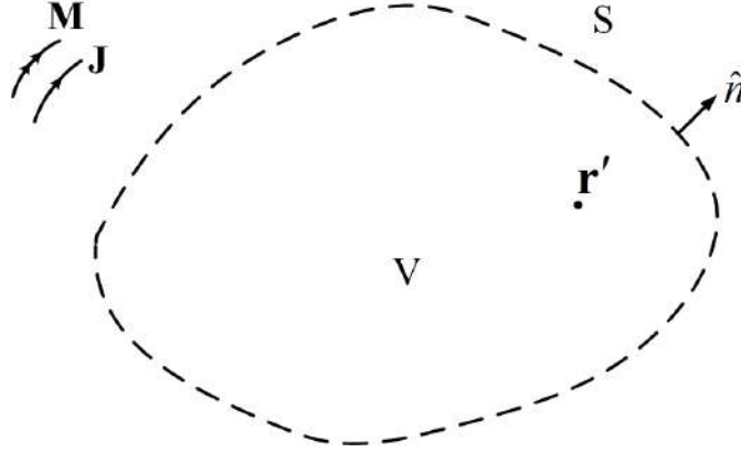
Figure 13.8: Derivation of the Huygens's principle for the electromagnetic case. One only needs to know the surface fields on surface S in order to determine the field at \mathbf{r}' inside V .
