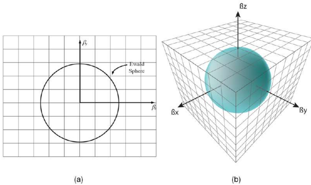
Figure 11.5: For a very large cavity, the grid spacing in the mode space (or Fourier space, also called the reciprocal lattice space [98, 99]) becomes very small. The radius of the sphere is given by \beta . Then the chance that the sphere surface encounters a resonant mode is very high. When this happens, the solution to the cavity problem is nonunique. (a) shows the 2D case while (b) shows the 3D case. The sphere defined by the equation \beta^2 = \beta_x^2 + \beta_y^2 + \beta_z^2 is known as the Ewald sphere. Here, k is equivalent to \beta .
