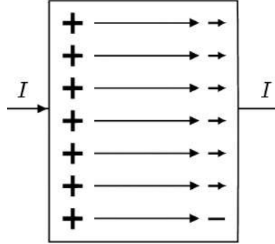
Figure 14.3: The schematic of the field inside a resistor. Due to charge accumulation, the potential on the left side is always higher than that on the right side. An electric field thus points from the left to the right inside the resistor.
