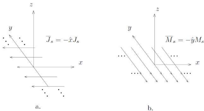
Figure 30.8: An infinite electric or magnetic current sheet, by the equivalence principle, can launch a perfect plane wave. The plane waves are propagating above and below the current sheet. [35, p. 653]
