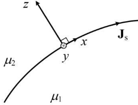
Figure 4.5: A figure showing the derivation of boundary condition for Ampère's law. A local coordinate system is used for simplicity.
