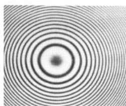
Fig. 2. Newton's rings
