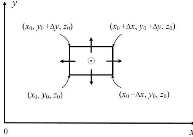
Figure 2.3: Illustration of the calculation of fluxes from a small cuboid where a corner of the cuboid is located at (x_0, y_0, z_0) . There is a third z dimension of the cuboid not shown and coming out of the paper. Hence, this cuboid, unlike that shown in the figure, has six faces.
