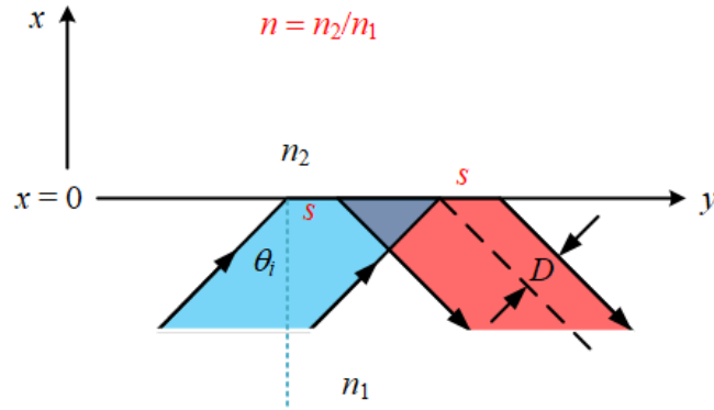
Figure 18.6: Goos-Hänchen Shift. A phase delay is equivalent to a time delay. In the time domain, one imagines a pulse traveling along a ray. When the ray hits the interface, it travels laterally on the interface for a distance s before being refracted back. The extra distance s traveled gives rise to the time delay (Figure by Paul R. Berman (2012), Scholarpedia [147]).
