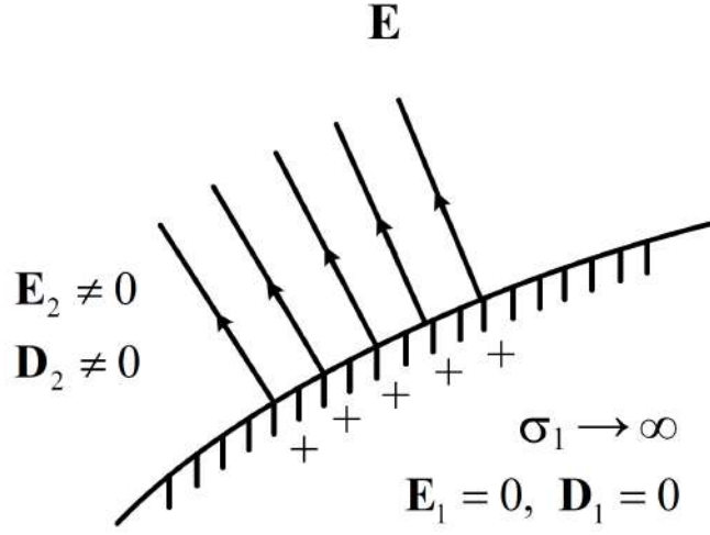
Figure 5.3: The behavior of the electric field and electric flux at the interface of a PEC and free space (or air).
