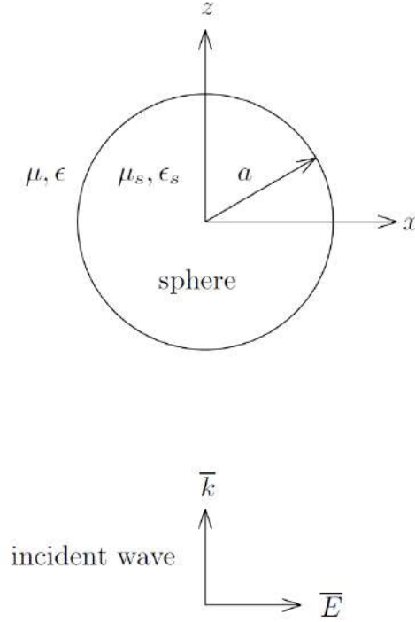
Figure 34.8: Geometry to illustrate the Mie scattering problem. The incident wave is traveling in the z direction so that it is symmetric about the z -axis, which simplifies the analysis. The problem can be solved in closed form using spherical harmonic expansions and Debye potentials.
