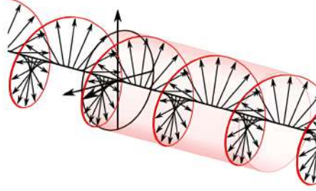
Figure 9.3: The rotation of the field vector of a RHCP wave as it propagates in the right direction [88]. (Figure by Wikipedia.)
