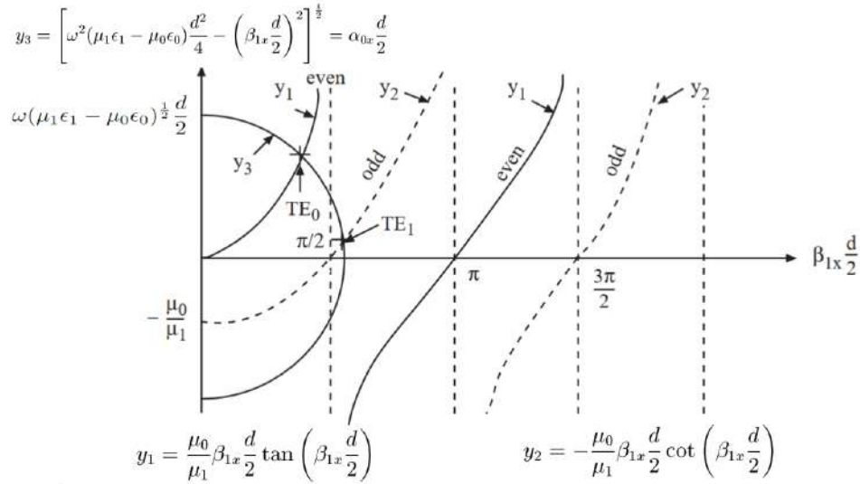
Figure 21.4: A way to solve (21.2.14) and (21.2.15) is via a graphical method. In this method, both the right-hand side and the left-hand side of the equations are plotted on the same plot. The solutions are at the intersection points of these plots.
