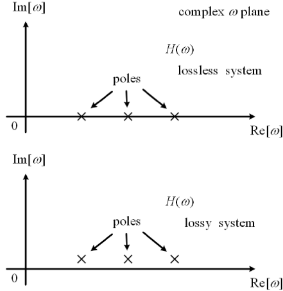
Figure 11.2: The nonuniqueness problem is intimately related to the locations of the poles of a transfer function being on the real axis, when one solves a linear system using Fourier transform techniques. because For a lossless system, the poles are located on the real axis, the Fourier inverse transform is not defined since the Fourier inversion contour is on the real axis. But when performing a Fourier inverse transform to obtain the solution in the time domain, then the Fourier inversion contour is undefined, and the solution cannot be uniquely determined.
