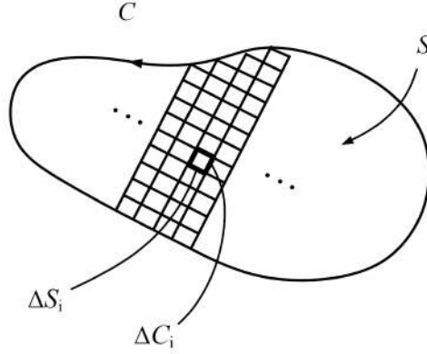
Figure 2.5: In proving Stokes's theorem, a closed contour C is assumed to enclose an open flat surface S . Then the surface S is tessellated into the sum of small rects (rectangles) as shown. The staircasing error at the boundary C vanishes in the limit when the rects are made vanishingly small.
