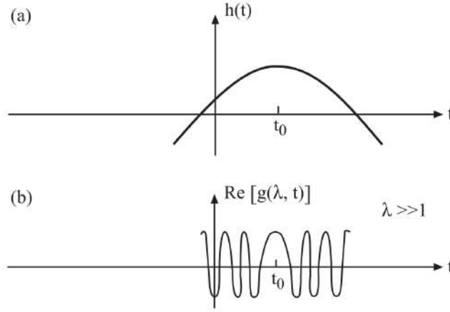
Figure 35.7: We first look at h(t) which is in the exponent of g(\lambda, t) (see (35.3.2)). Here, h(t) is a slowly varying function of t as shown in (a). But it is in the exponent multiplied by \lambda . When \lambda is large, the function g(\lambda, t) is rapidly varying where its real part is as shown in (b).
