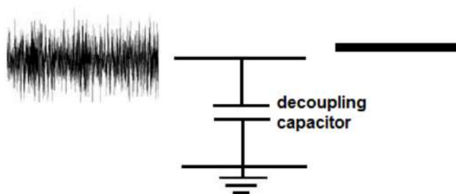
Figure 14.13: A decoupling capacitor is essentially a low-pass filter allowing low-frequency signals to pass through, while high-frequency signals are short-circuited (Figure by: https://www.ic-components.com/blog/a-comprehensive-guide-to-decoupling-and-bypass-capacitors-mechanisms,applications,and-differences.jsp ).
