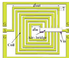
Figure 14.16: Spiral inductors are difficult to build on a chip, but by using laminal structure, it can be integrated into the IC fabrication process. The fabrication of circuit components has to be commensurate with the photolithography and chemical processes used (Figure by: researchgate.com, Quan Yuan).
