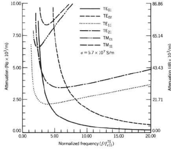
Figure 24.2: Plots of losses of different modes in a circular waveguide with a radius of 1.5 cm. It is seen that at high frequencies, the TE_{01} mode has the lowest loss (Figure by: C. A. Balanis and E. Holzman, “Circular waveguides,” Encyclopedia of RF and Microwave Engineering, 2005.).
