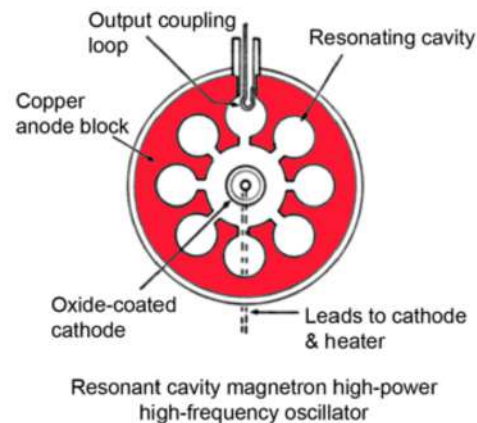
Figure 25.15: A magnetron works by having a high-Q microwave cavity resonator. When the cavity is injected with energetic electrons from the cathode to the anode, the kinetic energy of the electron feeds into the energy of the microwave. The cavity resonance amplifies this field-electron interaction, causing energy transfer from the kinetic energy of the electrons to the electromagnetic field energy (Figure by https://en.wikipedia.org/wiki/Cavity_magnetron [198]).
