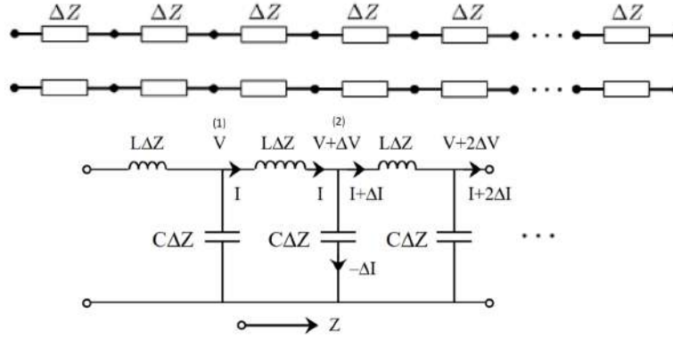
Figure 15.3: A long transmission line can be replaced by a concatenation of many short transmission lines. For each pair of short wires, there are capacitive couplings between them. Furthermore, when a current flows in the wires, a magnetic field is generated, making the wires behave like an inductor. Therefore, the transmission line can be replaced by a lumped-element approximation as shown. The lumped elements have inductances given by L\Delta z and capacitances given by C\Delta z , distributed over the line. This is also known as the distributive model of the transmission line. There were many lumped-element models of a transmission line, but the final one that captures the physics correctly is due to Heaviside [43].
