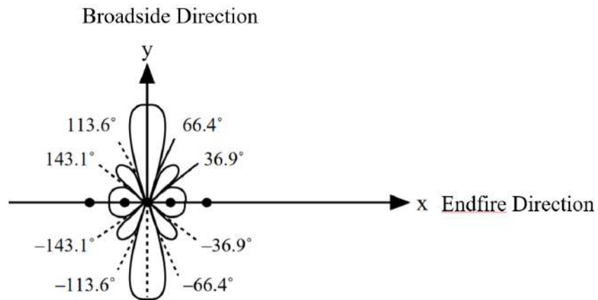
Figure 30.5: The radiation pattern of a five-element broadside array. These terms have descended from war ships. Assuming that the ship is traveling in the x direction, then the y direction is the broadside of the ship. The broadside and endfire directions of the array are also labeled.
