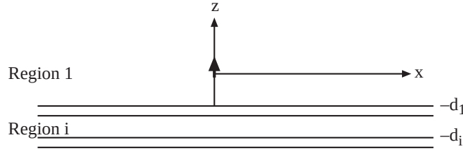
Figure 35.6: A vertical electric dipole over a layered medium.
