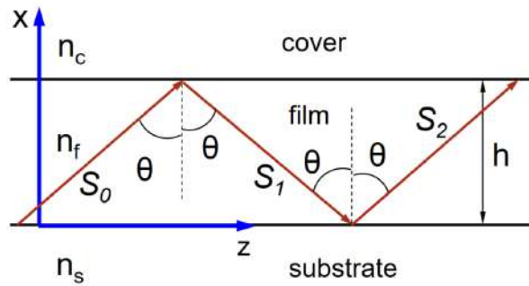
Figure 18.7: The total internal reflections (TIR) at the two interfaces of a thin-film waveguide can be used to guide an optical wave (Figure by E.N. Glytsis, NTUA, Greece [148]).
