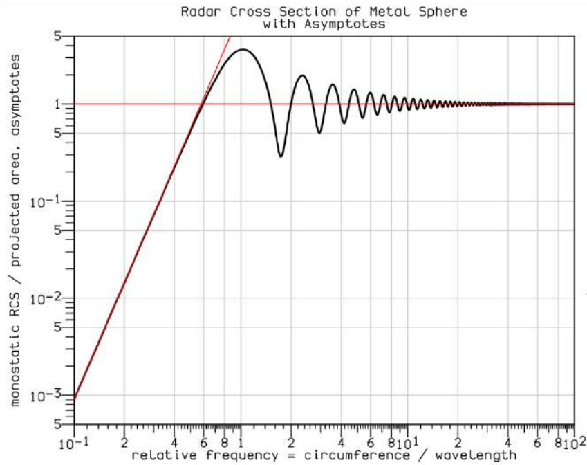
Figure 34.6: Radar cross section (RCS) calculated using Mie scattering theory (Figure by: https://www.researchgate.net ) [275].
