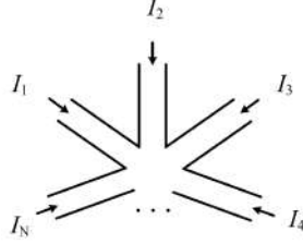
Figure 14.1: Schematic showing the derivation of KCL. All currents flowing into a node must add up to zero. This is reminiscent of the current continuity equation which is a statement of charge conservation. Viz., \nabla \cdot \mathbf{J}(\mathbf{r}) = -\partial_t \rho(\mathbf{r}) , which in the static limit, becomes \nabla \cdot \mathbf{J}(\mathbf{r}) = 0 .
