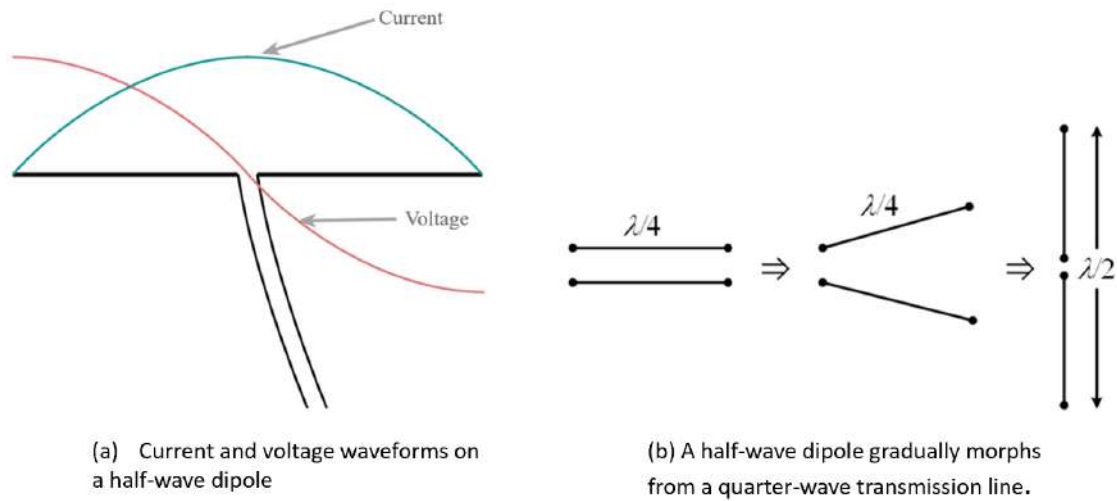
Figure 28.11: Approximate current distribution on a half-wave dipole (Figure by: electronics-notes.co). The currents are zero at the two end tips due to the current continuity equation, or KCL. A more precise calculation of its input impedance is given in [59].
