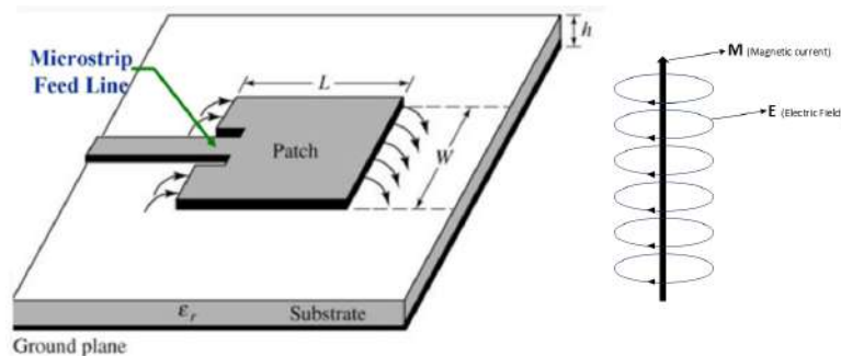
Figure 31.6: A microstrip patch antenna showing fringing electric fields at the two apertures. The fringing electric fields can be thought of as equivalent magnetic currents. The magnetic currents have the same E fields, and they can be used to model the radiation of the patch antenna (Figure by everthingRF.com).
