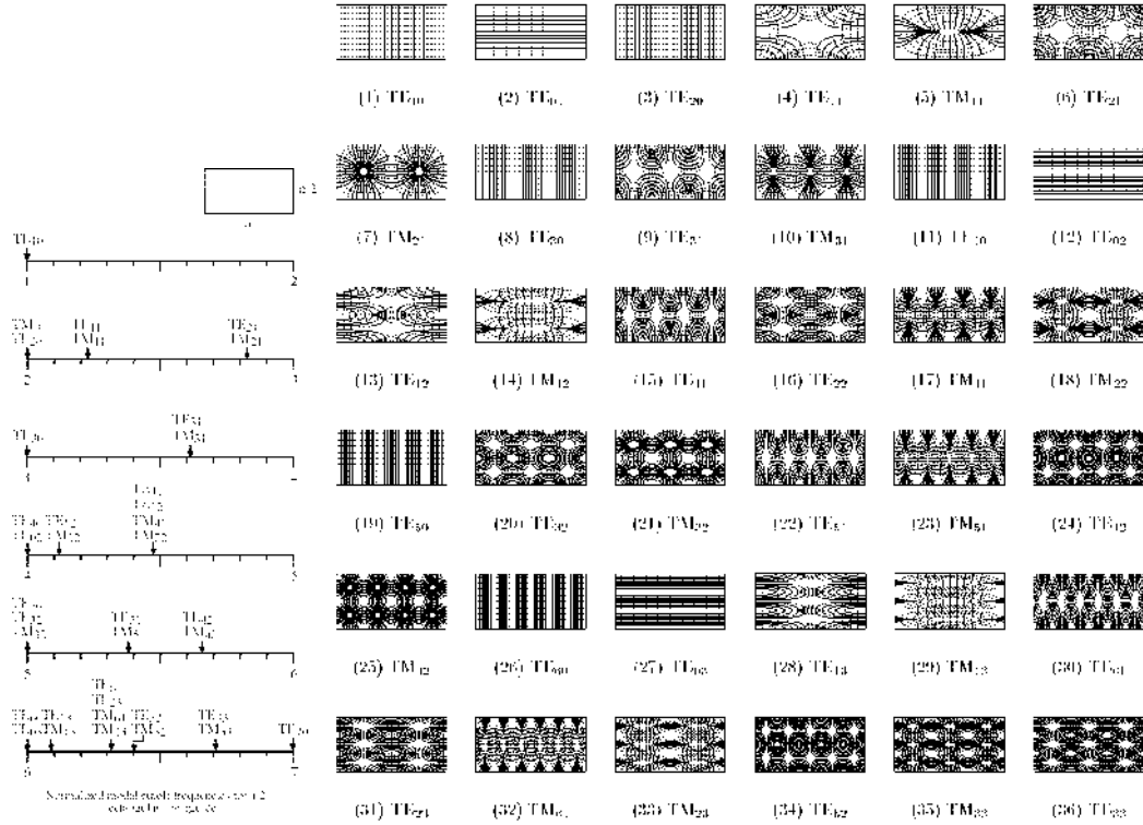
Figure 23.4: Transverse field plots of different modes in a rectangular waveguide (Figure by Andy Greenwood. Original plots published in Lee, Lee, and Chuang, IEEE T-MTT, 33.3 (1985): pp. 271-274. [178]).
