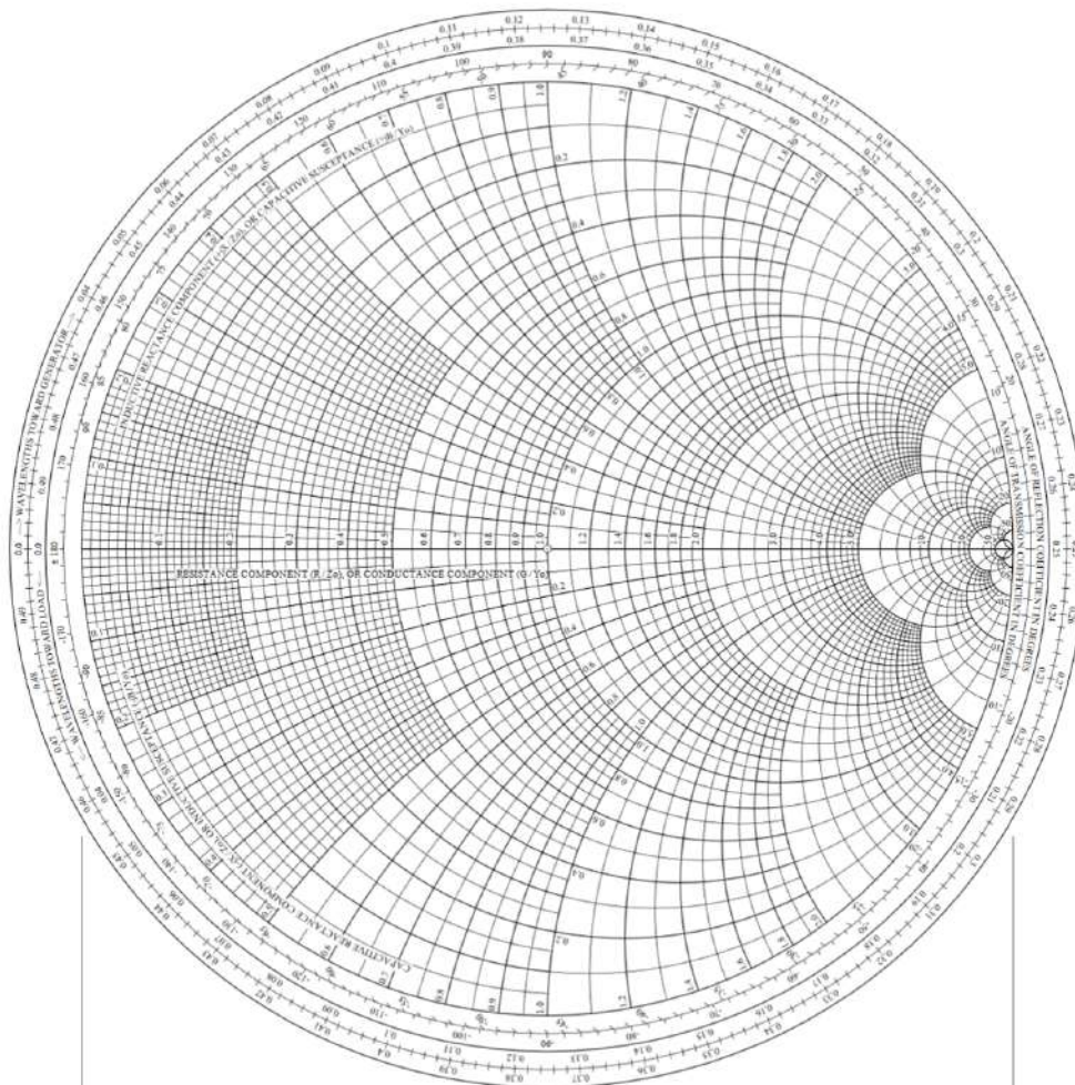
Figure 16.10: The Smith chart in its full glory. It was invented in 1939 before the age of digital computers, but it still allows microwave engineers to do mental estimations, gymnastics, and rough predictions with it. Because of its simplicity, it has an indelible influence on microwave engineering. (Figure by: https://en.wikipedia.org )
