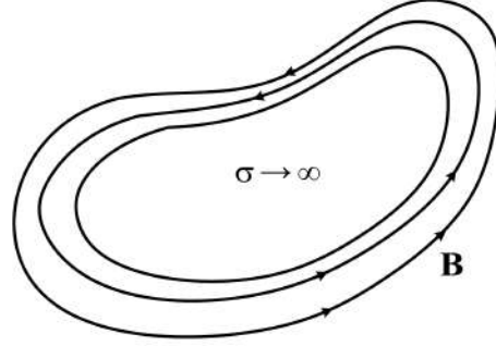
Figure 5.6: Sketch of the magnetic flux \mathbf{B} around a PEC. As explained in the text, it is seen that \hat{n} \cdot \mathbf{B} = 0 at the surface of the perfect electric conductor.
