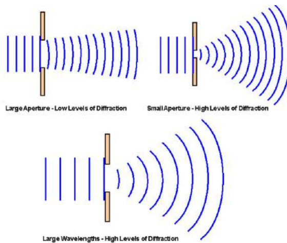
Figure 30.9: Diffraction of a plane wave by apertures of different sizes. The laser pointer works like diffraction of short wavelength plane waves by a large aperture. The beam remains like a plane wave after diffraction, and hence it is collimated for a Rayleigh distance before beam divergence sets in (Figure by imagen-estilo.com).
