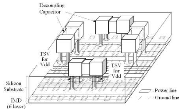
Figure 14.15: Modern computer chip design is 3D and is like an “urban jungle” like Manhattan or Hong Kong. There are different levels in the chip and they are connected by through-silicon vias (TSVs). IMD stands for intermetal dielectrics. One can see different XY lines serving as power and ground lines. Clever engineering has upheld the self-fulfilling prophecy of Moore’s law. Because of the complexity of modern chip designs, and the common electromagnetic interference between the components, signal integrity (SI) and power integrity (PI) are important issues in their designs (Figure by: springer.com).
