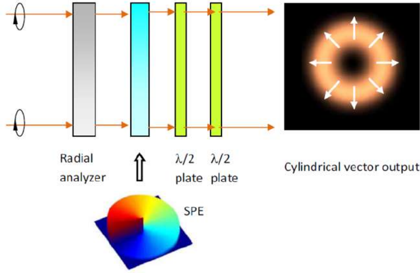
Figure 10.2: A cylindrical vector beam can be generated experimentally. The spiral phase element (SPE) compensates for the \exp(\pm j\phi) phase shift (Figure by: https://www.mdpi.com/2076-3417/10/10/3427 (Zhan Q.) [89]). The half-wave plate rotates the polarization of a wave by 90 degrees.
