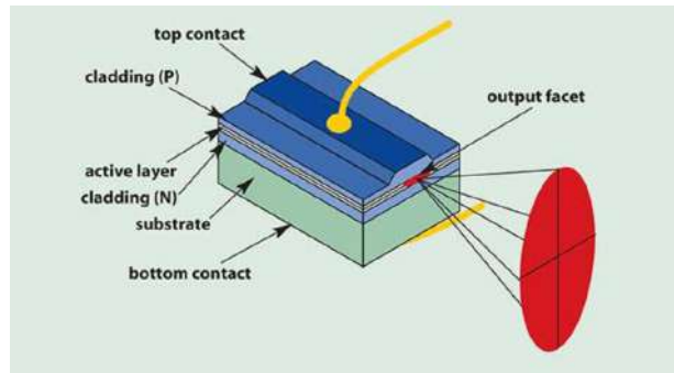
Figure 25.17: A semiconductor laser (also known as a laser diode) at work. Room temperature lasing is possible due to the tight confinement of both light photons and electron-hole pair carriers. Their close proximity causes the diode to lase at room temperature (Figure by: Photonics.com).
