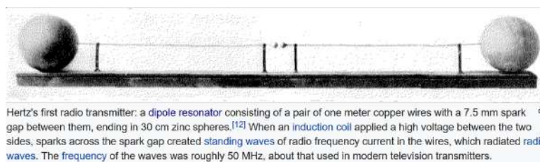
Figure 28.1: Hertz's original experiment on a small dipole (Figure by: H. Hertz, "On the finite velocity of propagation of electromagnetic actions," Electric Waves, vol. 110, 1888).
