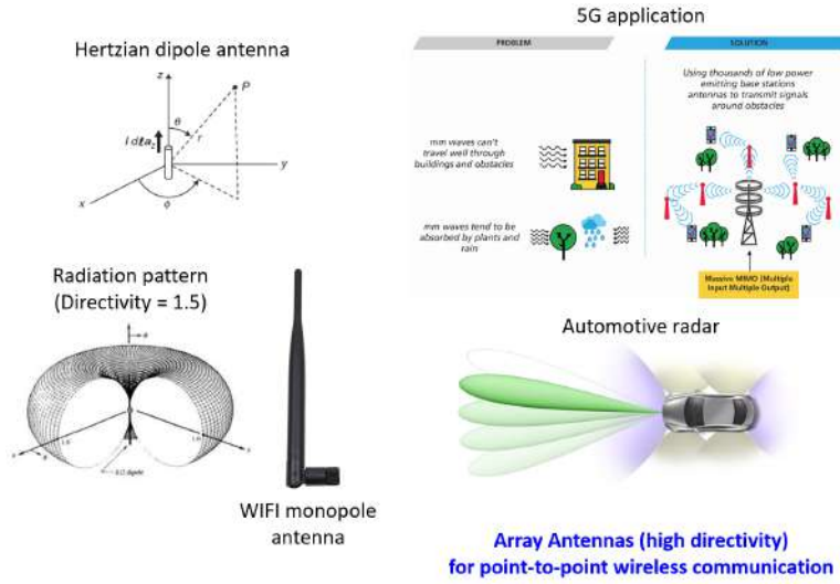
Figure 30.2: The left figures show the low directivity of a Hertzian dipole. The right figures show applications for which array antennas are needed to improve directivity and better communication links of a 5G communication system, which can operate as high as 54 GHz. The bottom right figure shows the collision avoidance system (CAS) of a car. The CAS of cars typically operate around 77 GHz so that the electromagnetic signals can penetrate through fog and rain (assembled by D.Y. Na).
