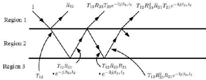
Figure 20.3: The expression of the generalized reflection coefficient decomposed into a ray series. Here, l_2 = d_2 - d_1 is the thickness of the slab (Figure by W.C. Chew [164]).
