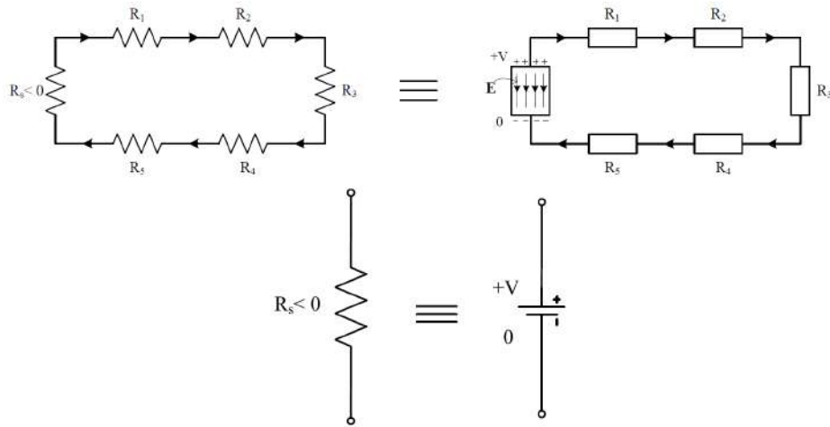
Figure 14.4: As shown above, a voltage source can also be modeled by a negative resistor.
