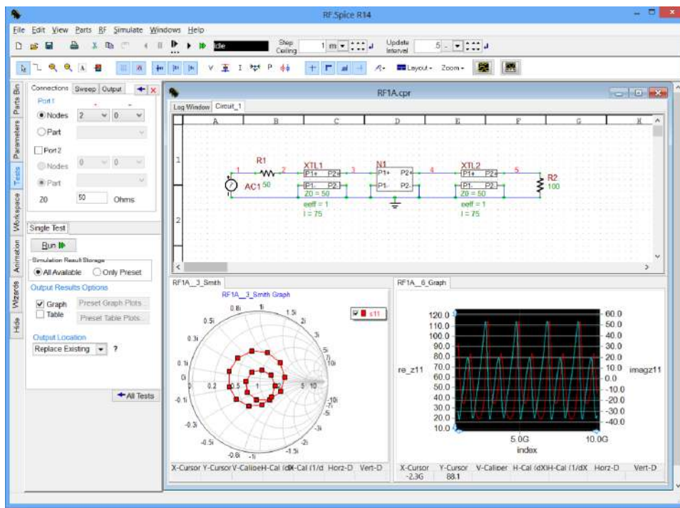
Figure 14.14: SPICE is also used to solve RF problems. A transmission line, to be discussed in the next lecture, is used in combination with circuit theory to account for retardation effects in a complex computer circuit (Figure by EMAG Technologies).
