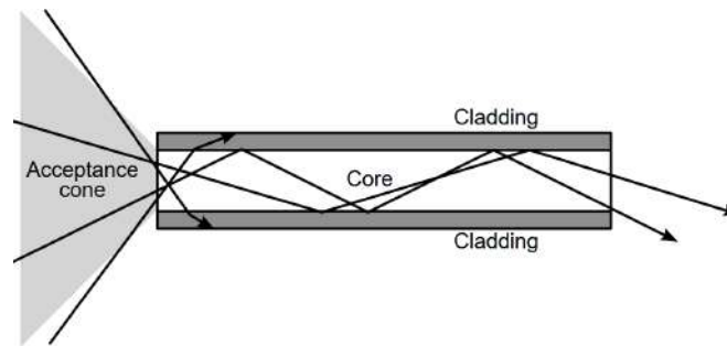
Figure 18.8: An optical fiber consists of a core and a cladding region. Total internal reflections (TIRs), due to phase-matching condition, can occur at the core-cladding interface. TIR can guide an optical wave in the fiber, which has a tremendous impact on the communication industry due to the low loss of the optical fiber (Figure by: https://www.researchgate.net [150]).
