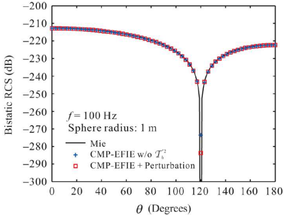
Figure 34.5: RCS (radar cross section) of a small PEC scatterer (Figure by Sheng et al. [273]). There is no true PEC in optics [215], but at RF and microwave, many conductors can be approximated by PEC.
