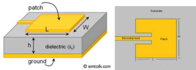
Figure 31.5: A microstrip patch antenna also radiates well when it resonates. The patch antenna resembles a cavity resonator with a magnetic wall [228]. Again, it uses the physics of resonant tunneling to enhance its radiation efficiency. The notch increases the length of the current flow and reduces the resonant frequency of the antenna (Figure by emtalk.com).
