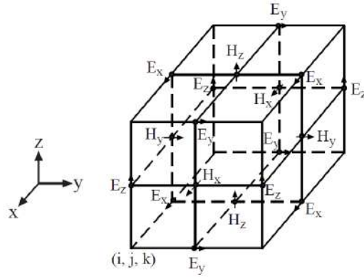
Figure 37.3: The assignment of fields on a grid in the Yee algorithm [308]. This algorithm is vastly popular for electromagnetic simulations [310].
