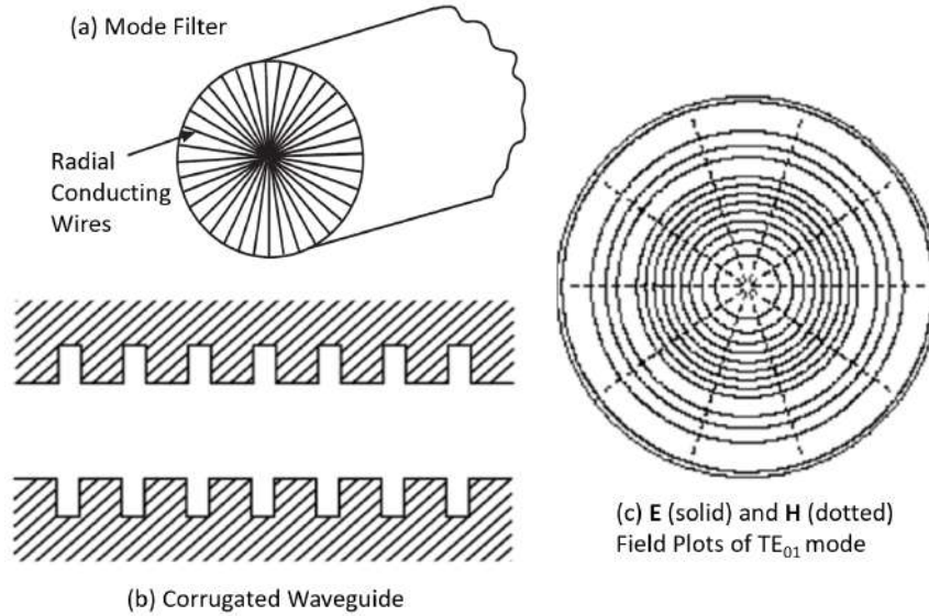
Figure 24.4: The TE_{01} has \mathbf{E} = \hat{\phi}E_{\phi} , and the tangential \mathbf{H} field only has a z component on the waveguide wall. Hence, the wall current is purely circumferential (azimuthal) for this mode. There are ways to enhance the TE_{01} mode in a circular waveguide: (a) use a mode filter that only allows the TE_{01} mode to go through or (b) use a corrugated waveguide to discourage axial current flow from the other modes but encourage the circumferential (azimuthal) current flow from this TE_{01} mode. The field plot of the mode is shown in (c). Such a waveguide is used in radio astronomy to design the communication links between antennas in a very large array (VLA [185]), or it is used in a circular horn antenna [186].
