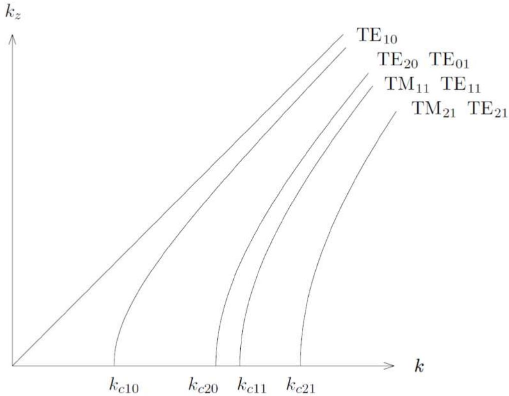
Figure 23.2: Dispersion curves for a rectangular waveguide (Figure by J.A. Kong [35]). Notice that the lowest TM mode is the TM_{11} mode, and that the TM_{mn} modes and the TE_{mn} modes have the same cutoff frequencies if they exist. Here, k is equivalent to \beta in this course. At cutoff, \beta_z = k_z = 0 , or the guided mode does not propagate in the z direction, and as shown above, the group velocity is zero. But when \omega \rightarrow \infty , the mode propagates in a direction almost parallel to the axis of the waveguide (this is called the “paraxial wave” in the parlance of wave physics), and hence, the group velocity approaches that of the waveguide medium.
