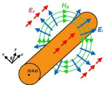
Figure 31.2: The electromagnetic field around a Goubau line (Figure by B. Vaughn and D. Peroulis, “An updated applied formulation for the Goubau transmission line,” Journal of Applied Physics , vol. 126, no. 19, p. 194902, 2019). The field resembles that of a coaxial line with the outer conductor (or ground) gradually moved to infinity. It can be thought of as a quasi-transmission line. When applied to a half-wave dipole, the mode is quasi-guided on the wire and is torn away from the wire antenna as it reaches its ends. Then it is launched into space at the end of the line.
