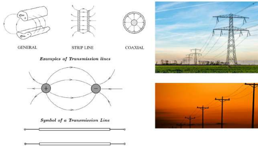
Figure 15.1: Various kinds of transmission lines. Schematically, all of them can be modeled by two parallel wires. On the right are pictures of a power transmission lines, and a telephone line. Due to technological advancements, telephone lines are a rare sight now (Figure by: Istockphoto.com).
