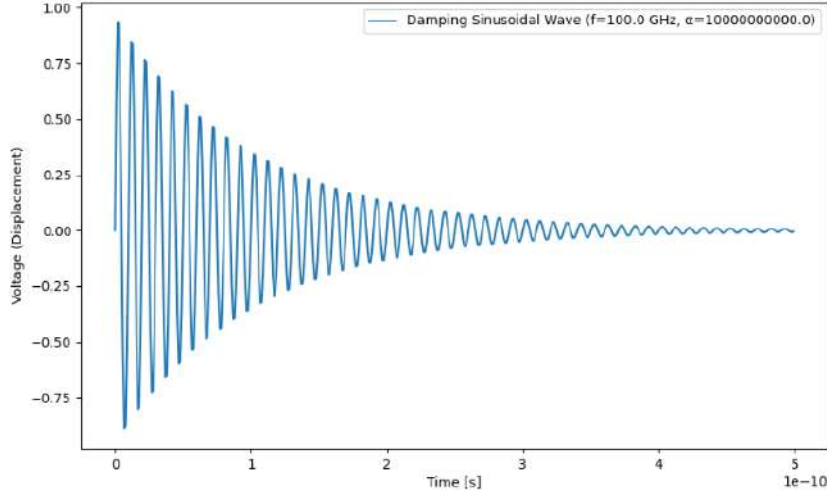
Figure 26.2: A typical time domain response of a high Q system.
