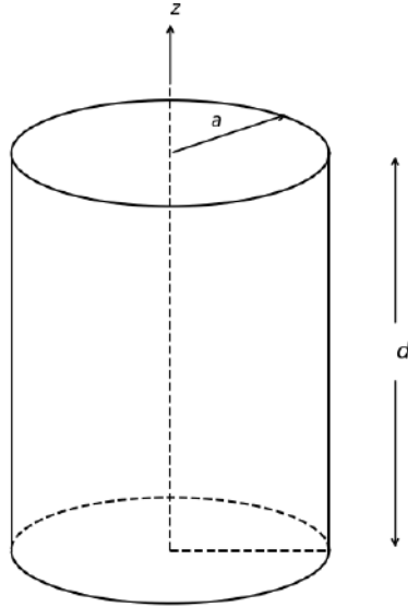
Figure 25.8: A circular resonant cavity made by terminating a circular waveguide at both ends.
