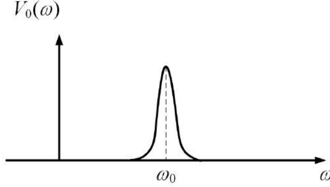
Figure 20.6: The frequency spectrum of V_0(\omega) is the Fourier transform of V(z = 0, t) (see (20.2.7)). As can be seen, it is a narrowband signal. Only with a narrowband signal can we define what a group velocity is. It is the velocity of the envelope of a pulse function.
