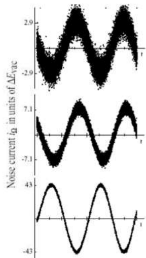
Figure 39.2: The time evolution of the coherent state at the very low average signal level. It is sinusoidal, but with great uncertainty innate in it when the energy of the coherent state is small (Figure By: https://en.wikipedia.org/wiki/Coherent_state ).
