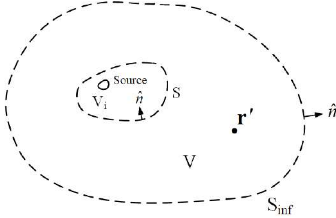
Figure 13.7: The geometry for deriving Huygens's principle for scalar wave. The radiation from the source can be replaced by equivalence sources on the surfaces S and S_{\text{inf}} , and the field inside V bounded by S and S_{\text{inf}} can be calculated using (13.4.5). Also, the field is zero inside S from (13.4.5). This is the extinction theorem. In other words, inside S , the field from the source is extinct by the field generated by the equivalent surface sources on S .
