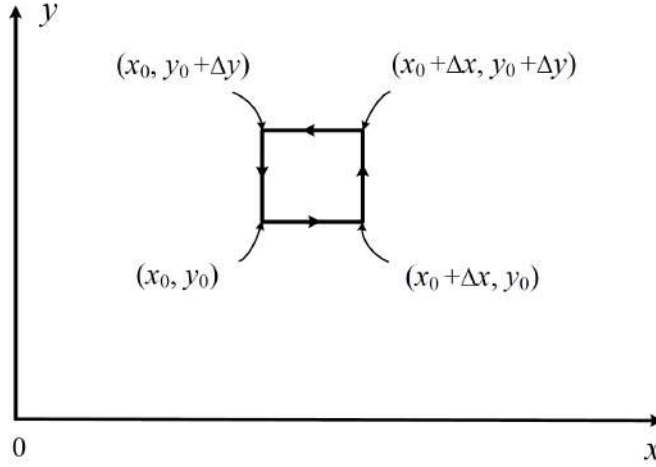
Figure 2.6: An approximation of the integration over a small rect. There are four edges to this small rect.
