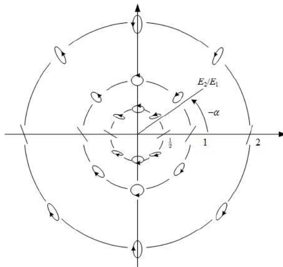
Figure 9.2: Due to phase differences between the E_x and E_y components of the field, and their relative amplitudes E_2/E_1 , different polarizations will ensue. The arrow indicates the direction of rotation of the field vector.
