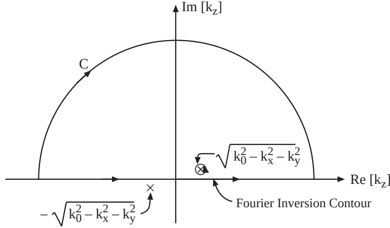
Figure 35.1: By invoking Cauchy's residue theorem, the integration along the real axis is equal to the integration along C plus the residue of the pole at k_z = (k_0^2 - k_x^2 - k_y^2)^{1/2} . By invoking Jordan's lemma, the integration around C is zero for most integrals, and thus, we require only the residue evaluation.
