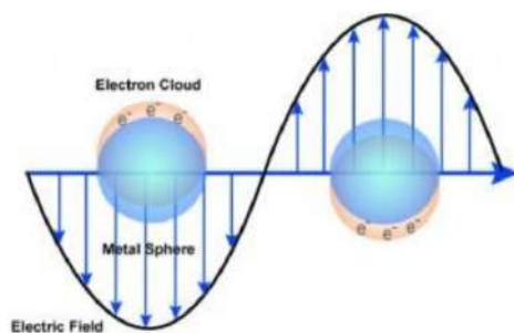
Figure 27.4: A nanoparticle undergoes electromagnetic oscillation when an electromagnetic wave impinges on it. The oscillation is inordinately large when the incident wave's frequency coincides with the resonance frequency of the plasmonic particle (Figure by sigmaaldric.com).
