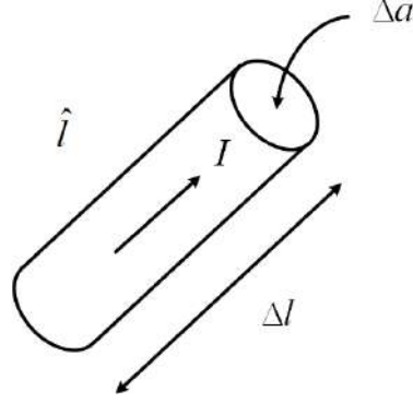
Figure 5.1: A current element used to illustrate the derivation of the Biot-Savart law. The current element generates a magnetic field due to Ampère's law in the static limit. This law was established experimentally, but here, we will derive this law based on our mathematical knowledge so far.
