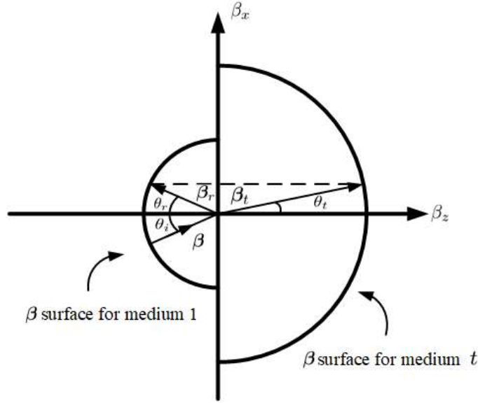
Figure 18.2: Wavenumber ( \beta or k ) surfaces in two regions showing the phase-matching condition. In this case, the wavenumber in medium t is larger (with larger \beta vector) than the wavenumber in medium 1. Then the wave vectors for the incident wave, reflected wave, and transmitted wave have to be aligned in such a way that their components parallel to the interface are equal because of the phase-matching condition. Also, one can see that Snell's law is satisfied as required by the phase-matching condition.
