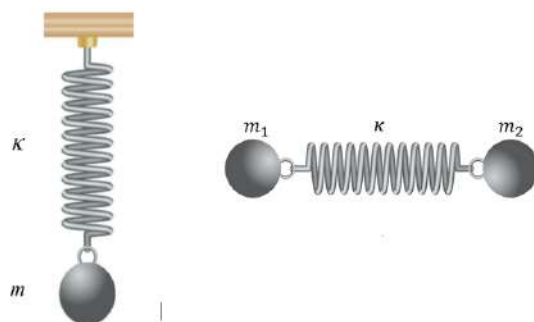
Figure 38.3: A classical pendulum can be used to illustrate classical Hamiltonian theory. The equation of motion of a classical pendulum can be derived using Newton's law or Hamiltonian theory. As such, it is easier to illustrate the quantum theory of a pendulum starting with classical Hamiltonian theory. In the figure, \kappa and m are spring constant and mass, respectively of the pendulum. The horizontal pendulum on the right can be simplified using the center-of-mass coordinate [339].
