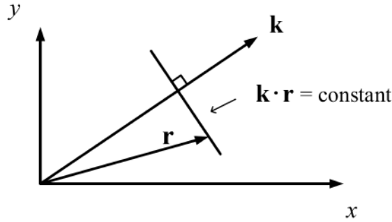
Figure 7.4: A figure showing the geometrical meaning of \mathbf{k} \cdot \mathbf{r} equal to a constant. It is a flat plane that defines the wavefront of a plane wave.
