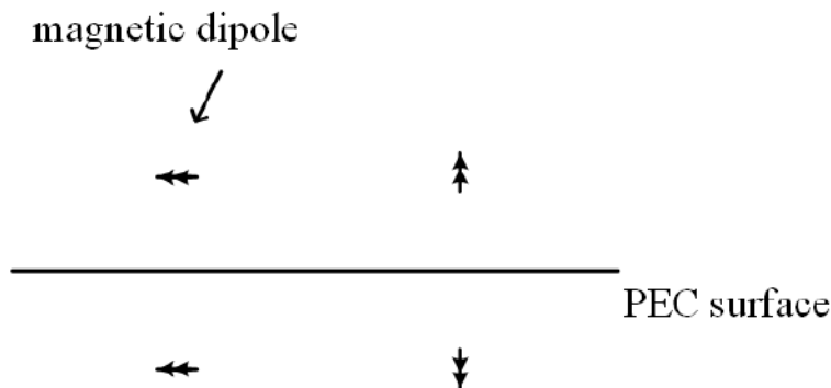
Figure 32.10: Using the rule of how a magnetic monopole reflects itself on a PEC surface, the reflection rules for magnetic dipoles can be ascertained. (Magnetic dipoles are often denoted by double arrows).
