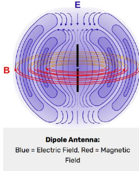
Figure 35.5: Sketch of the time-harmonic EM fields of a VED. The electric field resembles that of Figure 29.1(a) which is the electric field of a radiating dipole. Only part of the magnetic field is shown here (Figure by: Subsonic.ae).
