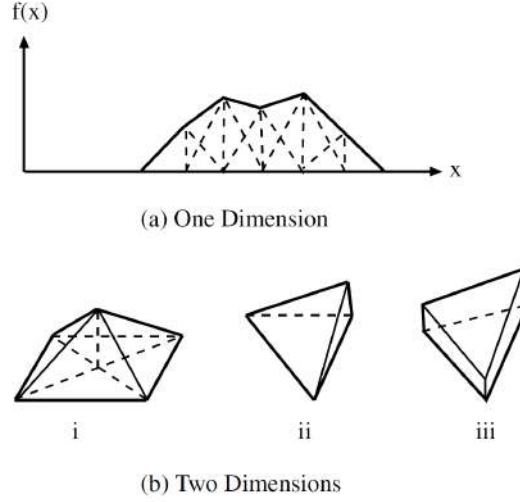
Figure 36.6: Examples of basis function in (a) one dimension; and in (b) two dimensions. Each of these functions are defined over a finite domain. Hence, they are also called subdomain basis functions. They can be thought of as interpolatory functions where the values in between the nodes are obtained by interpolation of the nodal values. When generalized to 3D, these basis functions become tetrahedrons, which are harder to draw and visualize.
