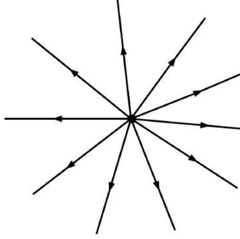
Figure 1.6: Emanating \mathbf{E} field from an electric point charge as depicted by (1.3.9) and (1.3.10). The physical meaning of the figure is that, a positive charge q is placed at the center.
