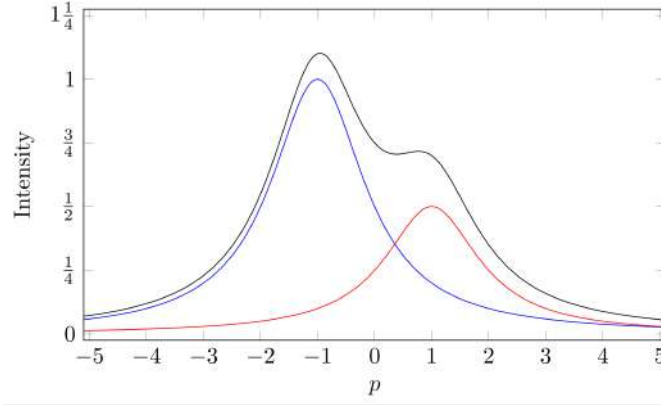
Figure 8.4: A Lorentzian function has almost a bell-shaped curve. By assuming multispecies of DLS oscillators in a medium, one can fit absorption spectra of almost any shape. (Figure by: https://commons.wikimedia.org ) ([77]).
