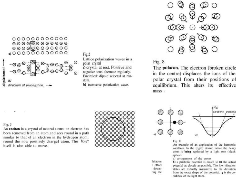
Figure 8.2: These figures are from Quantum Field Theory of Solids by H. Haken. They provide a heuristic explanation of the electromagnetic property of solids (Figure by: Hermann Haken [75]).
