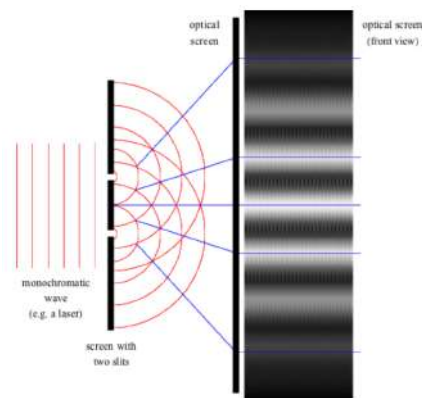
Figure 38.1: A Young's double-slit experiment. Again, the interference pattern reveals the wave nature of light (Figure By: https://www.shmoop.com ).
