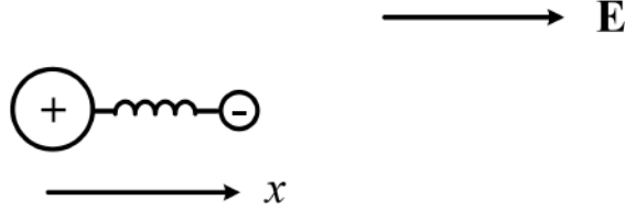
Figure 8.3: The electron with an effective mass is bound to the ion by an attractive force. This can be approximately modeled by a spring providing a restoring force to the electron.
