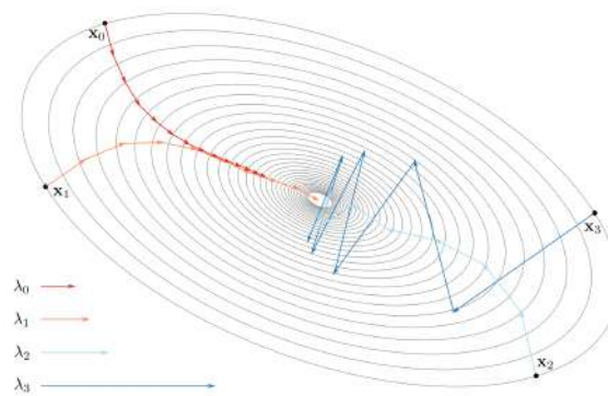
Figure 36.10: Gradient search or gradient descent method is finding an optimal point. As is obvious, the initial value is instrumental in converging into the correct solution (Figure by: Y. Ioannou, https://blog.yani.io/sgd/ ).
