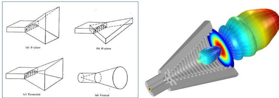
Figure 31.7: A horn antenna works under the same principle as the biconical antenna. Its flared horn changes the waveguide impedance to match the impedance of a waveguide to the impedance of free space. The right figure is that of a corrugated circular horn antenna. The corrugation enhances the propagation of the TE_{01} mode in the circular waveguide, and thus it enhances the cylindrical symmetry of the mode and the radiation field (Figure by: tutorialpoints.com and comsol.com).
