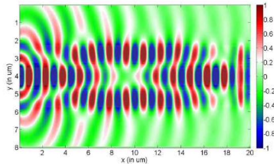
Figure 37.4: The 2D FDTD simulation of complicated optical waveguides. Such simulations can be done from static to optical frequencies (Figure by: https://www.mathworks.com ).
