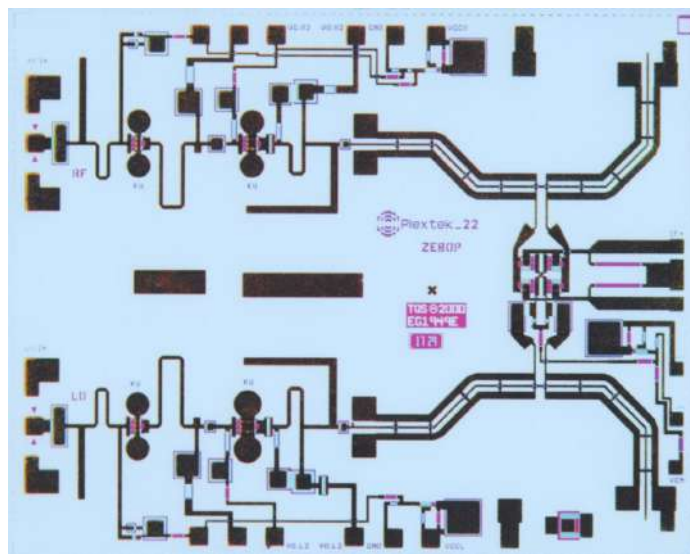
Figure 17.2: A generic GaAs MMIC. They are the motivation for studying multijunction transmission lines (Figure by: https://commons.wikimedia.org ).
