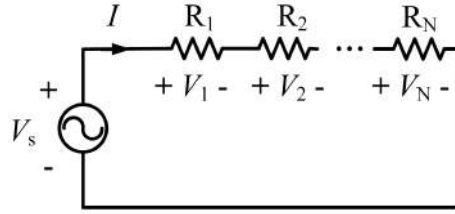
Figure 14.2: KVL where the sum of all voltages around a loop is zero, which is the consequence of static Faraday's law.
