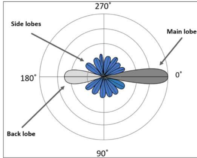
Figure 29.6: The directive gain pattern of an array antenna. The directivity is increased by constructive interference among the elements of the array antenna (Figure by Wikimedia).
