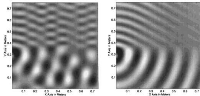
Figure 37.8: Simulation of a source on top of a half-space (left) without stretched coordinates PML ABC; and (right) with stretched coordinates PML ABC [327]. One can see the effect of standing wave patterns due to the reflections from the walls of the simulation domain. The reflected waves give rise to interference patterns that are clearly visible in the left figure. They disappear upon the introduction of stretched coordinates PML ABC (Figure by: https://www.semanticscholar.org/paper/Complex-coordinate-stretching-as-a-generalized-Chew-Jin/ff8da6ca4ad2358016ec169ffa43cb871873a842 ).
