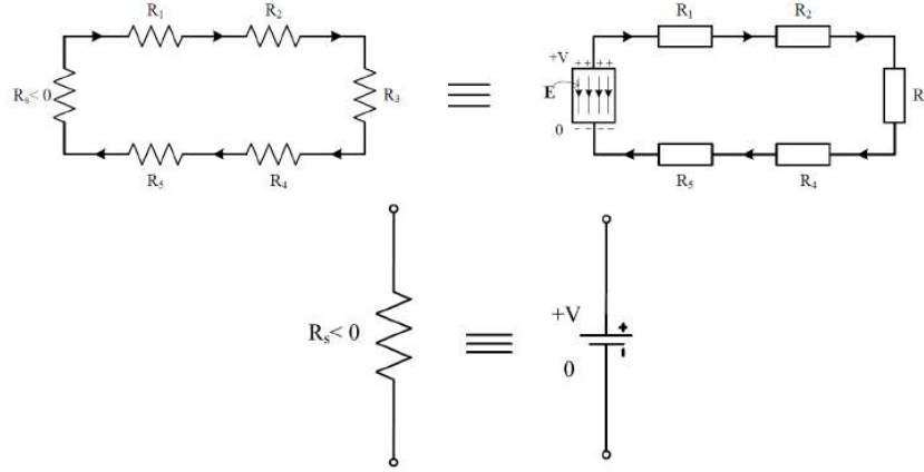
Figure 5.8: The dissipation of energy as the current flows around a loop. A battery can be viewed as having a negative resistance.
