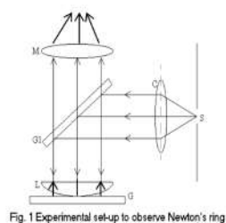
Fig. 1 Experimental set-up to observe Newton's ring
