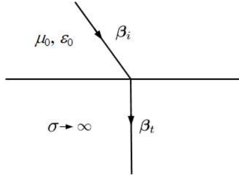
Figure 26.5: Due to high \sigma in the metal and large |\beta_t| , phase-matching condition requires the transmitted wave vector to be almost normal to the surface. Then the field can be assumed to be a normally incident plane-wave field in the transmitted or the metal region. The tangential electric field is almost zero, and the tangential magnetic field remains almost unchanged using this perturbative concept.
