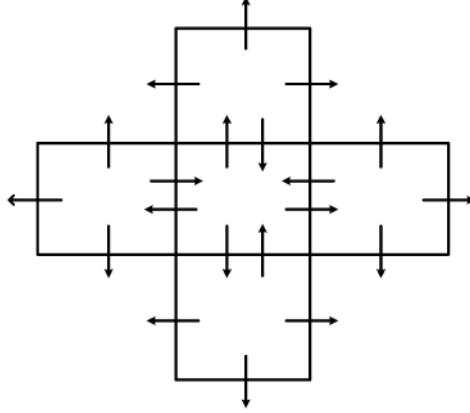
Figure 2.2: Fluxes from adjacent cuboids cancel each other, leaving only the fluxes at the boundary, that remain uncanceled. Please imagine that there is a third dimension of the cuboids in this picture where it comes out of the paper.
