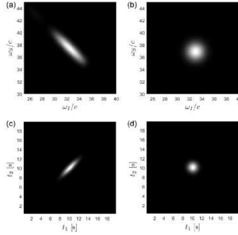
Figure 39.4: Spectral probability amplitudes for (a) two entangled photons and (b) two nonentangled photons. The degree of two-photon coincidence count rate or (c) entangled and (d) nonentangled photon pairs. The entangled photon pairs have both strong temporal correlation and frequency anti-correlation, but not for the non-entangled photon pairs [375].
