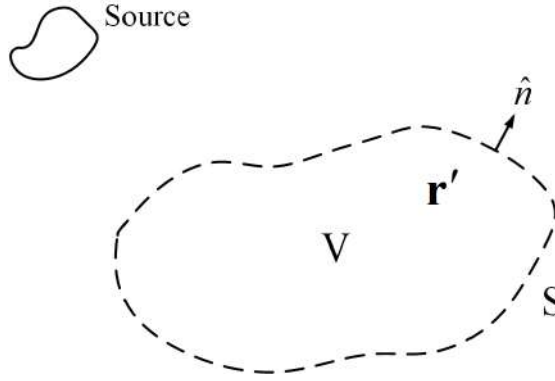
Figure 13.6: The geometry for deriving Huygens's principle for scalar wave equation. The dashed surface represents an “imagined” surface.
