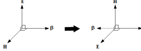
Figure 17.10: The unusual swap expounded in (17.2.12), though leaving Maxwell's equations unchanged, seems to disobey the right-hand rule for \mathbf{E} , \mathbf{H} , and \beta . But one can change the sign of \beta (as it is not unique) to obey the right-hand rule again.
