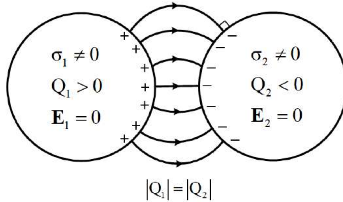
Figure 5.4: The behavior of the electric field and flux outside two conductors in the static limit. The two conductors need not be PEC, and yet the fields are normal to the interface, and the fields are zero inside them.
