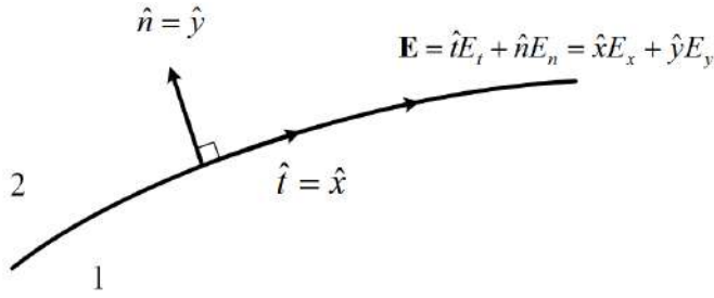
Figure 4.2: This figure is for the derivation of the boundary condition induced by Faraday's law. A local coordinate system can be used to see the boundary condition more lucidly. Here, the normal \hat{n} = \hat{y} and the tangential component \hat{t} = \hat{x} .
