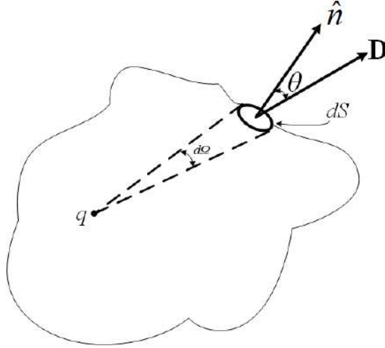
Figure 1.7: Electric flux through an incremental surface dS where \hat{n} is the unit normal and \mathbf{D} is the electric flux density passing through the incremental surface.
