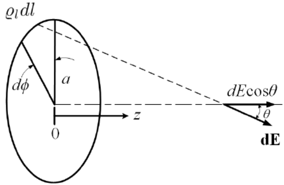
Figure 1.11: Electric field of a ring of charge (Figure by Ramo, Whinnery, and Van Duzer [34]).
