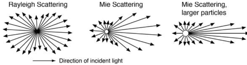
Figure 34.7: A particle scatters increasingly more in the forward direction as the frequency increases (Figure by: hyperphysics.phy-astr.gsu.edu).
