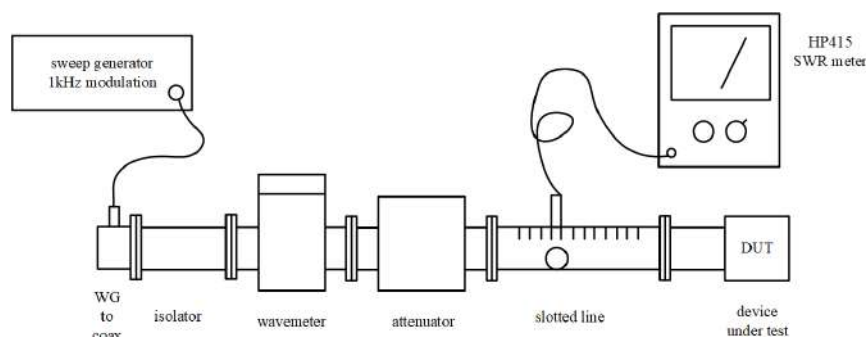
Figure 16.8: An experimental setup for a slotted-line measurement (Figure by: Pozar and Knapp, U. Mass [126]).
